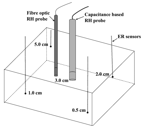
Fig. 3. The layout of the sensors in a limestone block.
