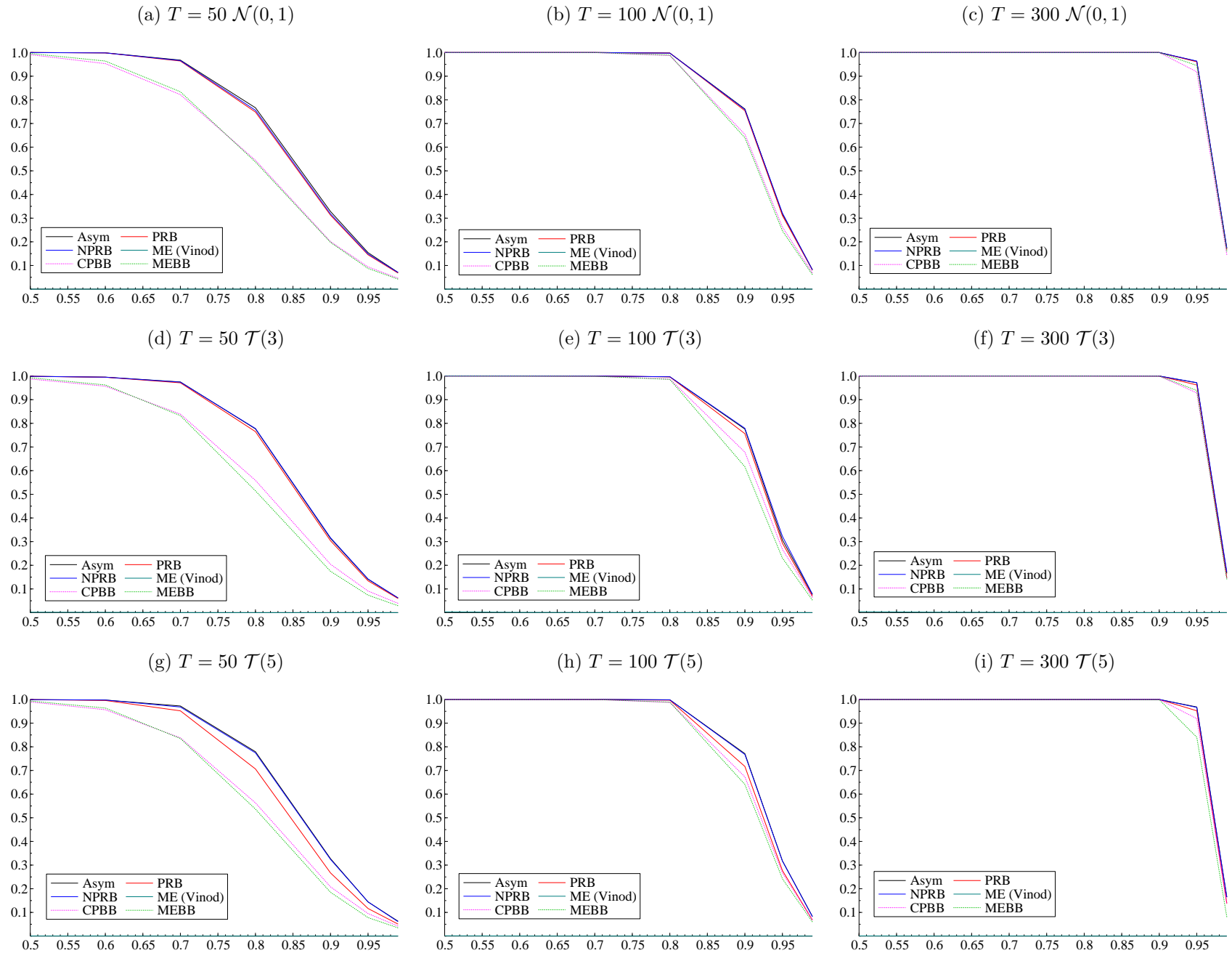
Figure 9: Power of the tests.
