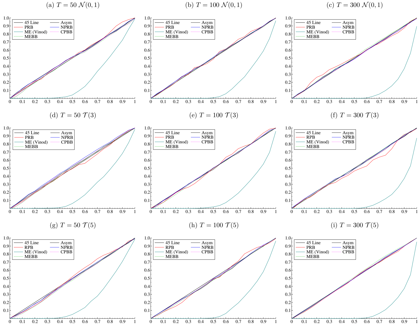
Figure 8: Empirical rejection frequencies.
