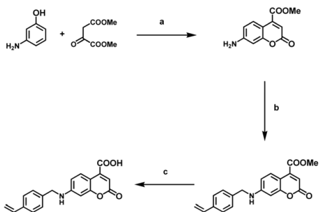
Scheme 1. Preparation of fluorescent monomer 7-VBACC. (a) 110 °C, 2 h, 42%; (b) CH 2 = CHC 6 H 4 CH 2 Cl, K 2 CO 3 , KI, MeCN, 85 °C, 50 h, 44%; (c) 1 M NaOH, EtOH/THF (2:1), 50 °C, 12 h, 94%.
