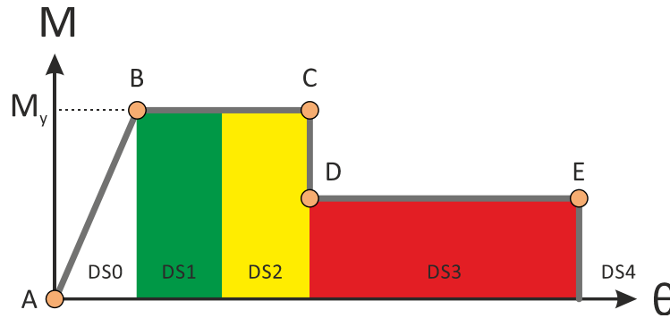
Fig. 12 Definition of damage states
