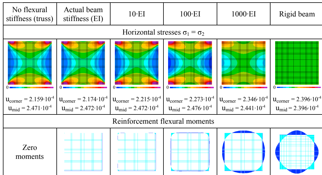
Figure 15. Parametric investigation on the effect of flexural rigidity of reinforcement bars.
