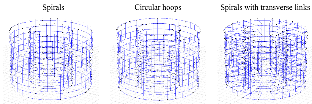
Figure 11. Various transverse reinforcement arrangements for circular sections.
