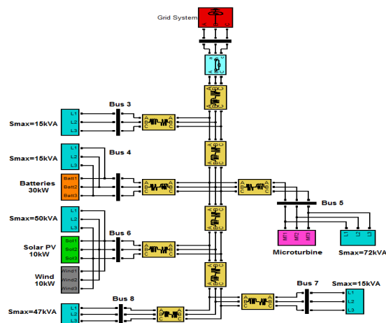
Figure 5. Benchmark LV microgrid networks using neural controllers.
