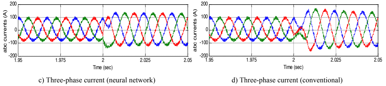
Fig. 1. Performance of PQ-inverter DER using conventional and neural network controllers ( T_s=1ms ).
