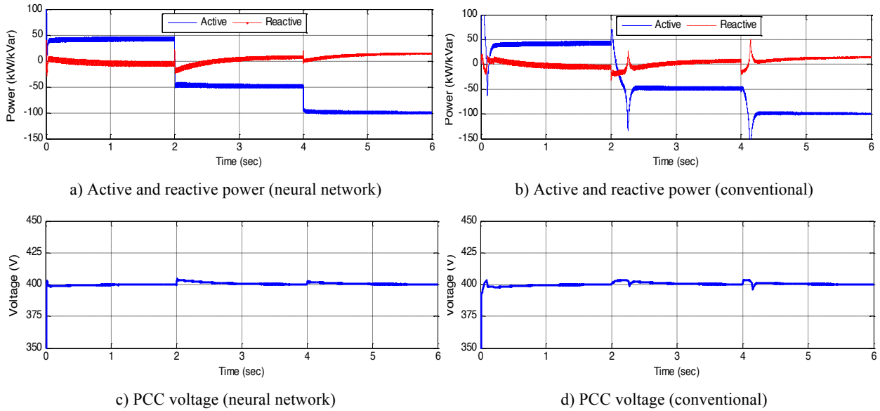
Fig. 2. Performance of PV-inverter DER using conventional and neural network controllers ( T_s=1ms ).
