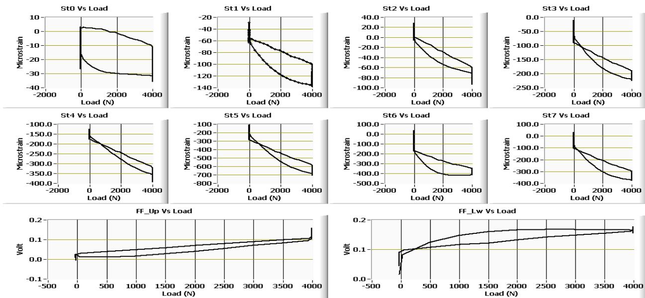
Fig.3: Exp1: 0-4-0@500NPS&LH300S; All eight strain gauge's outputs and two piezoresistive-Flexiforce® sensor's outputs with respect to applied compressive load in Newton.
