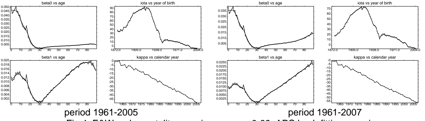
Fig 4. E&W male mortality experience, ages 0-89. APC back-fitting exercise. Reduction factor parameter patterns, with beta parameter smoothing.
