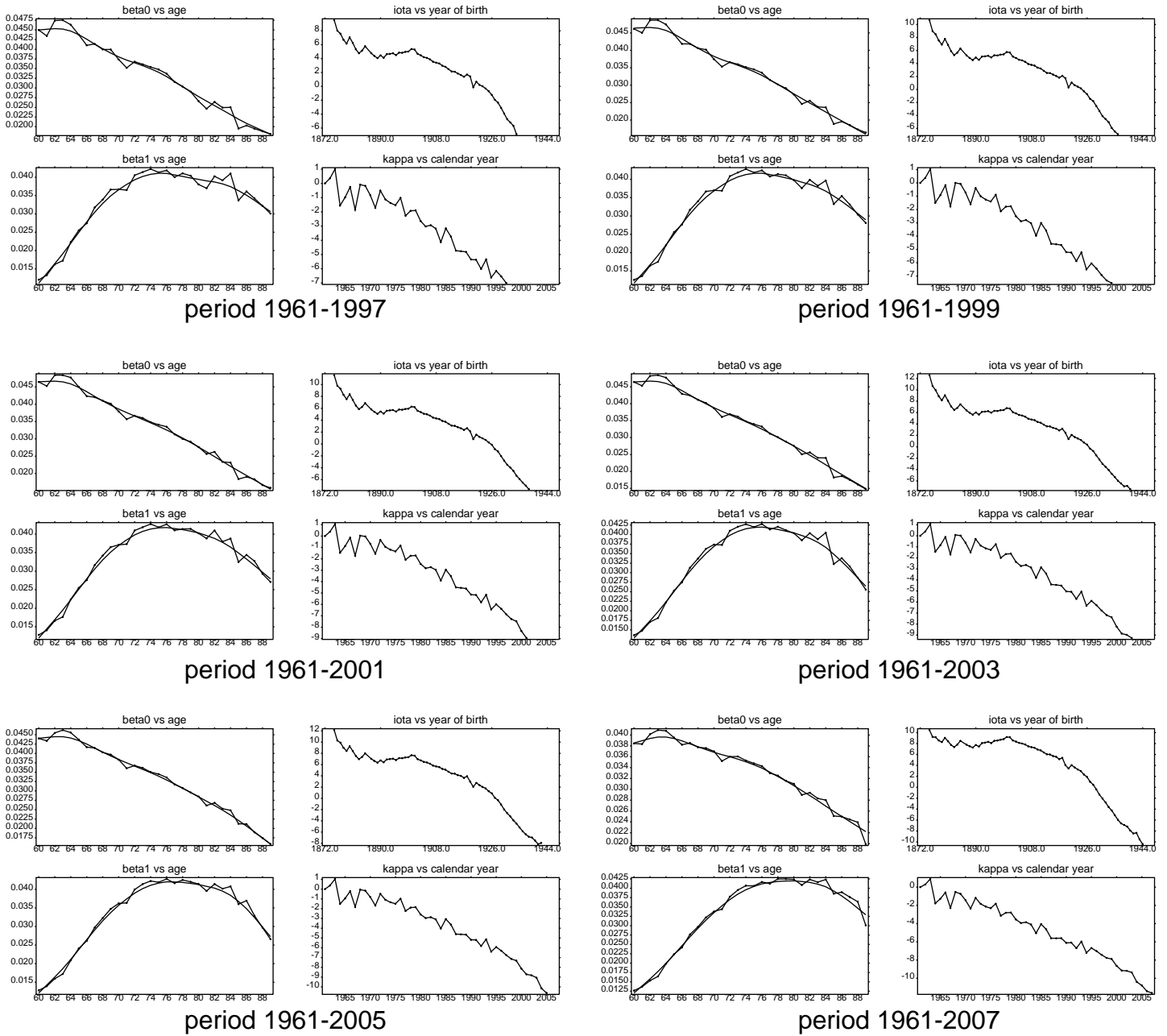
Fig 3. E&W male mortality experience, ages 60-89. APC back-fitting exercise. Reduction factor parameter estimates, with beta parameter smoothing.
