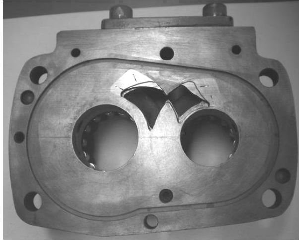
Figure 5 Modified shape of the discharge port
