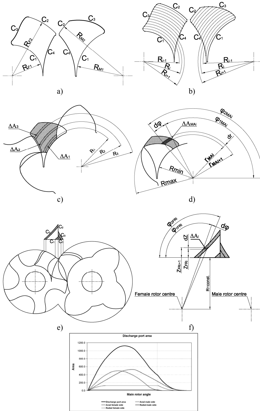
g) Figure 3 Principle of the discharge port area calculation
