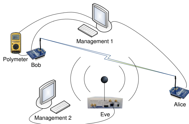
Figure 3: Test-bed topology
