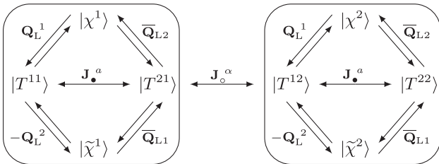
FIG. 2. The two massless \mathfrak{psu}(1|1)_{\text{c.e.}}^4 multiplets, in the representation (q_L \otimes \tilde{q}_L)^{\oplus 2} . Overall we have four bosons T^{a\alpha} and four fermions \chi^\alpha, \tilde{\chi}^\alpha , where a and \alpha are fundamental indices of \mathfrak{su}(2)_\circ and \mathfrak{su}(2)_\bullet . Again we show only some supercharges. Note that \mathfrak{su}(2)_\circ relates the two \mathfrak{psu}(1|1)_{\text{c.e.}}^4 modules.
