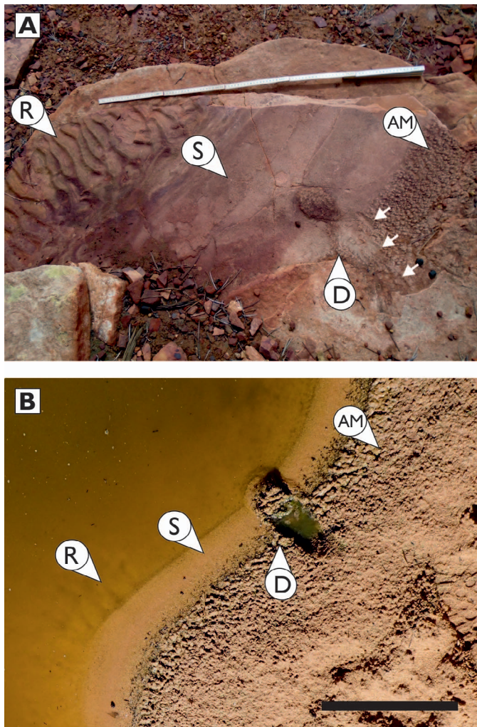
FIG. 6.—Evidence for preservation of primary sedimentary surface textures in the geological record, shown through comparison of ancient and modern surfaces. A) Bedding plane exposure of the Silurian Tumulagooda Sandstone, preserved in the wall of the Murchison River Gorge at The Loop. Ruler for scale is 1 meter. B) Modern pond of standing water in the Murchison River, west of The Loop. Scale bar = 20 cm. Both the modern and ancient examples reveal analogous substrate conditions, exhibiting ripple formation in deeper parts of a submerged pond (arrow R), a smooth substrate on the recently emergent drainage slope at the pond margin (arrow S), adhesion marks on the emergent margin of the pond (arrow AM), and a dislodged raft of adhesion marked sediment (arrow D). In the modern example, the raft was dislodged artificially, while in the ancient example it appears to have been dislodged by an arthropod; arthropod tracks are common in the formation and a series of grooves (small white arrows) at this location may be repichnial.
