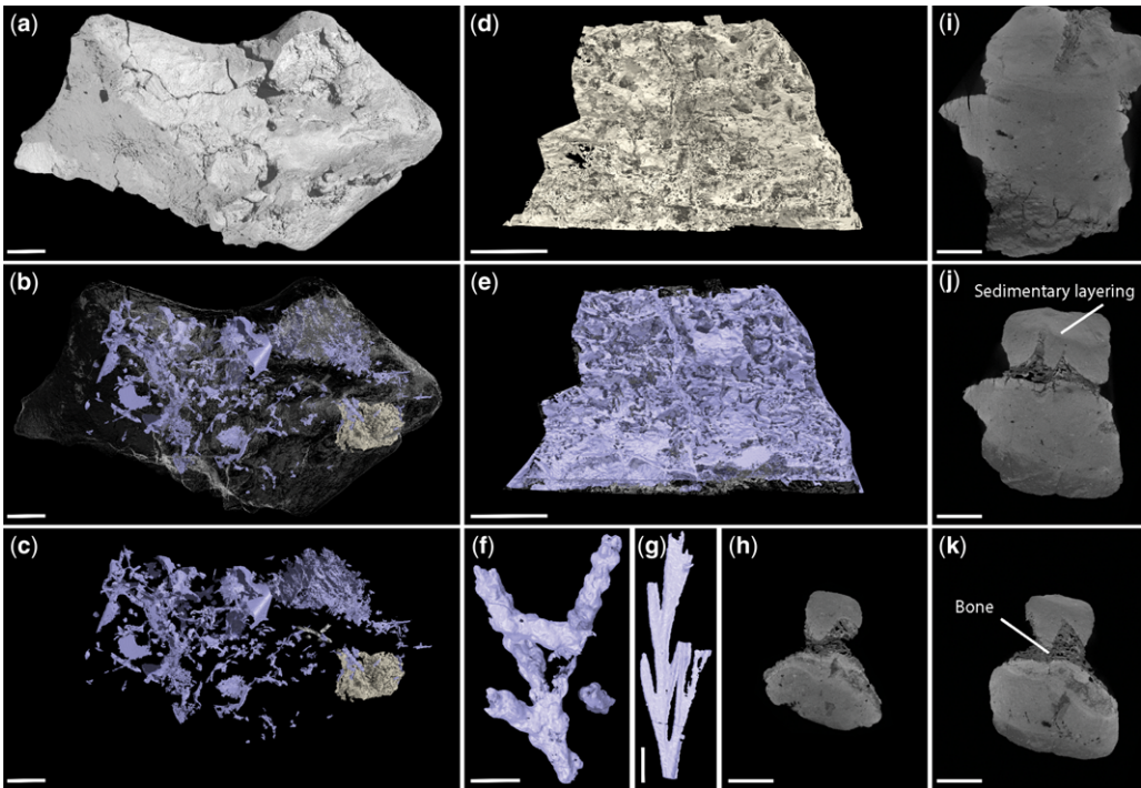
Fig. 5. Computed tomography reconstructions of: (a) the endocast (lateral view from the right side); (b, c) voids/regions of lower density within the endocast; (d) a bone fragment at the back of the endocast (dorsal view); (e) the voids within the bone fragment (interpreted as Haversian canals or trabeculae); (f) a branching twig within the sediment infill; and (g) a leaf within the sediment infill. (h–k) Representative computed tomography slices through the endocast revealing regions of bone and layering within the sediment infill. All reconstructions in this figure were generated using the SPIERS software suite and were rendered in Blender. Scale bars: (a–c, h–k) = 10 mm, (d, e) = 5 mm, (f, g) = 2 mm.
