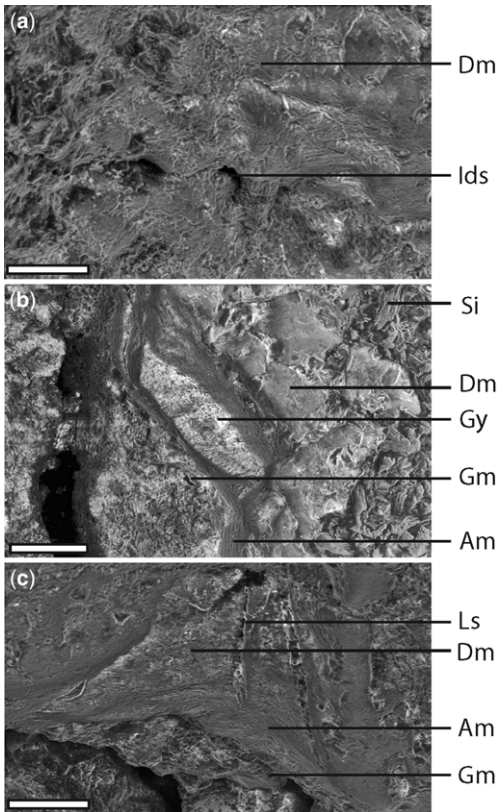
Fig. 6. Environmental scanning electron microscopy images of the iguanodontian natural cranial endocast. Images of the outer laminar layer on the flanks of the cerebellar area. (a) Well-preserved textures reflecting the organization of the meningeal layers lying immediately above the cortex; the pit-like structures represent intradural spaces lying between the thicker ribbons of meningeal tissue. (b) Features interpreted as folds and valleys of the meninges, lying above a complex fabric with recesses (Gy) possibly representing some of the superficial features of the underlying grey matter (Gm) of the cerebellar cortex. (c) Features interpreted as fossilized dura mater (Dm), the outermost membranes that surround the brain. Scale bars = 100 \mu\text{m} . All images in this figure were obtained from scans of the uncoated complete brain endocast. Am, probable arachnoid mater (traces of collagenous sheets and ribbons reinforcing the meningeal layer); Dm, probable dura mater preserved as micron-sized phosphatized filaments; Gy, potential gyri – these structures are normally associated with deeper layers in the cortex (i.e. the grey matter) and reflect some of the convolutions near the surface of the cortex; Ids, intradural spaces; Ls, lesions in the meningeal fabric; Si, lozenge-shaped siderite crystals.
