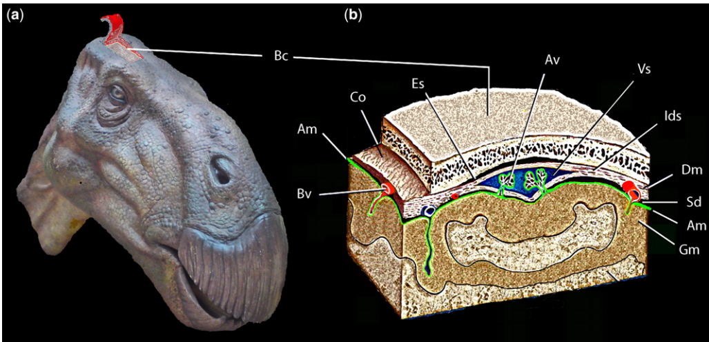
Fig. 9. An idealized reconstruction of the head of an iguanodontian dinosaur showing the dorsal braincase and associated soft tissue features as evidenced by examination of the natural endocast from Bexhill. (a) Reconstruction of the head of an iguanodontian (OUMNH T.127) in the oblique anterior view showing the area of the skull roof that has been 'dissected' to the right. (b) Partly 'exploded' restoration of the underlying braincase and brain tissues identified following detailed examination of the structures preserved in the natural cranial endocast. Am, arachnoid mater (meninge); Av, arachnoid villus (protruding into a mid-line venous sinus); Bc, braincase bone (parietal); Bv, blood vessels; Co, collagenous sheath enclosing the brain structures and lining the bones of braincase (combined periosteal and meningeal sheets); Dm, dura mater (meninge); Es, epidural space; Gm, grey matter (brain cortex); Lds, intradural space (between the meninges); Sd, subdural space; Vs, sagittal venous sinus.
