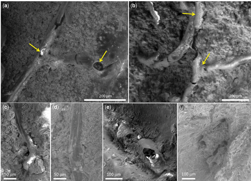
Fig. 7. Environmental scanning electron microscopy images of tubular structures on the exterior of the Bexhill iguanodontian cranial endocast and within the outer laminar layer, interpreted here as meningeal blood vessels. Arrows in (a) point to areas where the hollow nature of the vessels can be seen; arrows in (b) point to branching of the vessels; (c–f) additional images of hollow tubular structures within the outer laminar layer. All images in this figure were obtained from scans of the uncoated complete brain endocast.
