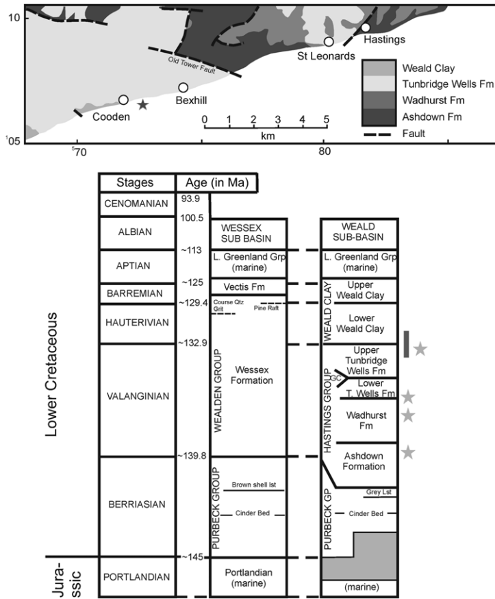
Fig. 1. Map and stratigraphic columns showing the geological context for the iguanodontian brain endocast, adapted from Brasier et al. (2009, fig. 1). Geological sketch map of the Bexhill area (Sussex, UK) follows that of Lake & Shephard-Thorn (1987), whereas the column and dates are updated and adapted after Allen & Wimbledon (1991) and Batten (2011). The endocast was discovered at a locality (black star) lying within the Upper Tunbridge Wells Formation. However, it was found ex situ and therefore may have a provenance from either the Tunbridge Wells Formation or the Lower Weald Clay (grey bar in stratigraphic columns). Grey stars indicate levels at which amber has been found (cf. Brasier et al. 2009, fig. 1).
