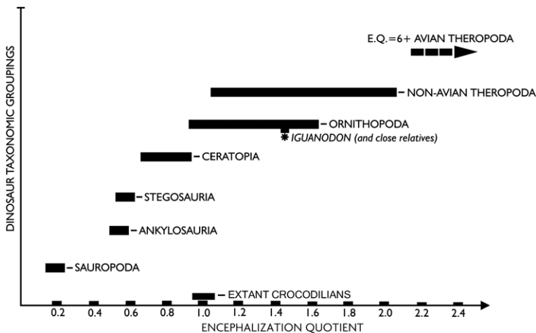
Fig. 10. Encephalization quotients (EQ) estimated across a range of dinosaur clades/groupings. Extant crocodylians represent the reference marker (EQ = 1.0) for comparison with dinosaurians more generally. Ornithopods (such as Iguanodon and closely related taxa) exceed the EQ of extant crocodylians and overlap the values seen in basal (non-avian) theropods. Modified from Hopson (1979).
