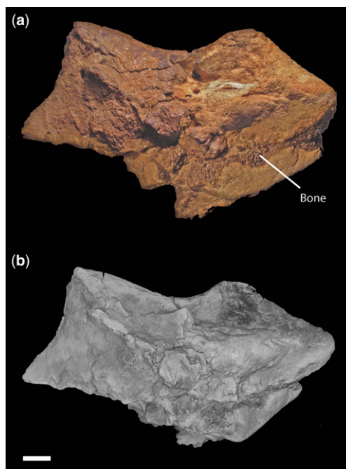
Fig. 3. Images of (a) the Bexhill iguanodontian natural endocast specimen and (b) a computed tomography volume render reconstruction of the same specimen viewed from the same orientation, made using Drishti. Scale bar = 10 mm. In the Drishti image, highly mineralized sections appear as more solid regions.
