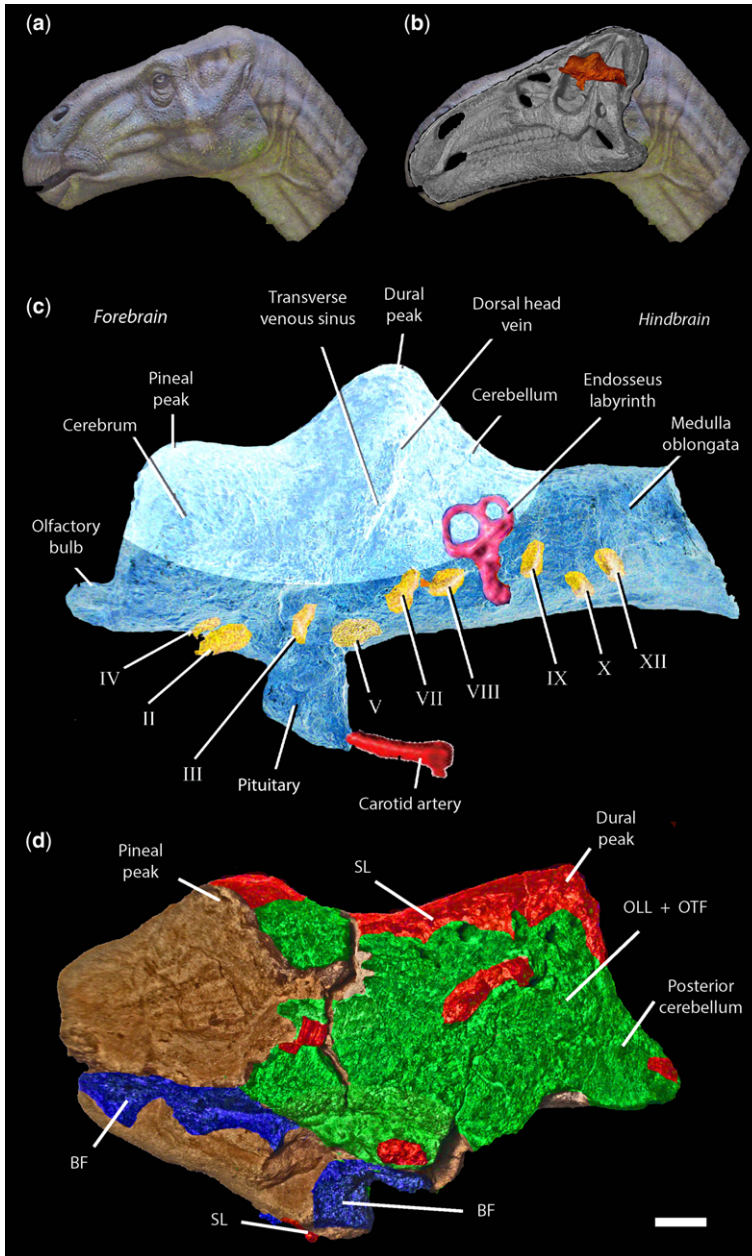
Fig. 2. Biological context for the iguanodontian endocast from Bexhill. (a) Life-like restoration of the head and anterior neck based on the anatomy of the iguanodontian ornithomimid Iguanodon bernissartensis (Norman 1980; OUMNH T.127). (b) Semi-transparent restoration of I. bernissartensis head showing the position and general morphology of the endocranial cavity (orange). (c) Interpreted image of the plaster cast of the endocranial cavity of Mantellisaurus cf. atherfieldensis (see also Supplementary material fig. 1a). The region in pale blue indicates the approximate extent of the natural endocranial cast described herein. The principal anatomical features and positions of brain-related tissues are indicated. Roman numerals indicate the positions of the principal cranial nerve canals, which have been superimposed with reference to earlier work by Norman (2004). (d) Natural cranial endocast with a false-colour overlay showing bone fragments (BF) in blue, a superficial layer (SL) of crystalline siderite (red) and an outer laminar layer (OLL) and outer tubular features (OTF) preserved in calcium phosphate (collophane; green). Natural colour = silty sediment.
