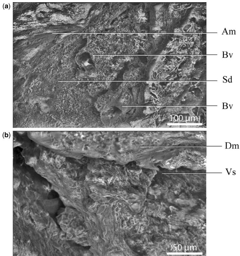
Fig. 8. Scanning electron microscopy images of small-scale tubular features and associated structures and fabrics visible on the outer laminar layer of the Bexhill iguanodontian natural cranial endocast. All images in this figure were obtained from scans of the uncoated complete brain endocast. Am, arachnoid mater-like fabric; Bv, tubular structures interpreted as blood vessels; Sd, fabric interpreted as dura mater; Vs, groove interpreted as a venous sinus.
