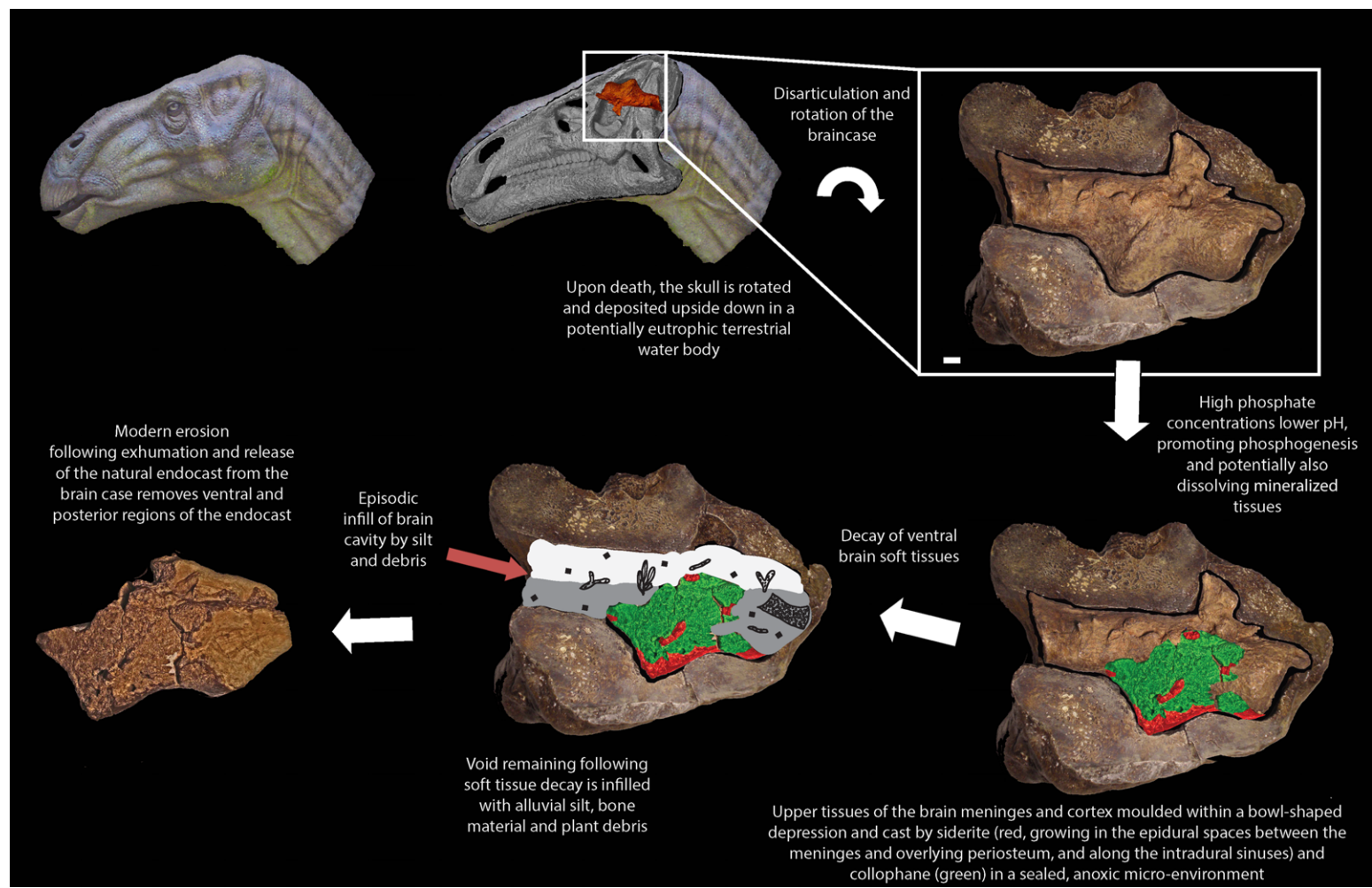
Fig. 4. A time sequence outlining the inferred taphonomic history of the iguanodontian natural endocast from Bexhill. Scale bar = 10 mm.
