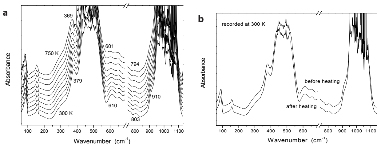
FIGURE 1. (a) Temperature evolution (in 300–750 K) of infrared spectra in the FIR and MIR regions (60–1130 \text{cm}^{-1} ) on heating. The temperature interval is 50 K. The spectra are offset for clarity. (b) Comparison of FIR and MIR spectra recorded at 300 K before and after heating to 780 K. The spectral similarities before and after the heating indicate that the temperature of 780 K is not high enough to cause irreversible structural changes (such as dehydroxylation).
