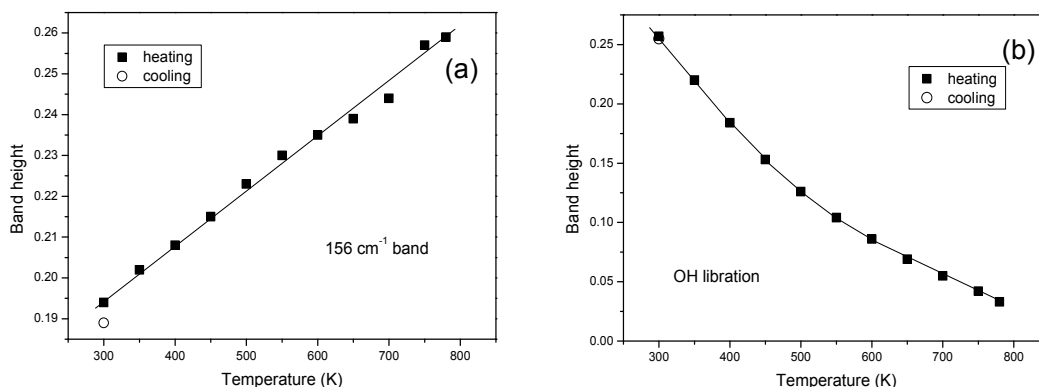
FIGURE 3. Band height as a function of temperature: (a) K–O band near 156\text{ cm}^{-1} , and (b) OH libration near 610\text{ cm}^{-1} .
