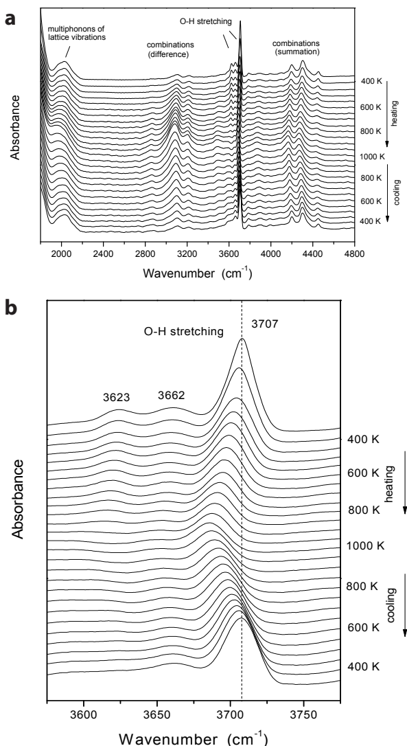
FIGURE 4. Temperature evolution of NIR spectra on heating and cooling (a) in the range 1800–4800 \text{cm}^{-1} and (b) enlarged section of the OH stretching region (in the range 3575–3775 \text{cm}^{-1} ). The spectra are offset for clarity.
