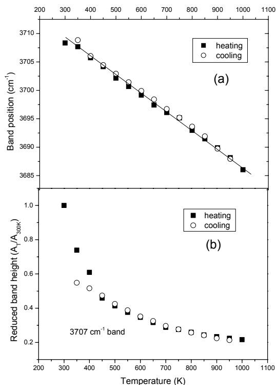
FIGURE 8. (a) Band frequency and (b) area of the 3707 \text{cm}^{-1} OH stretching vibration as a function of temperature.
