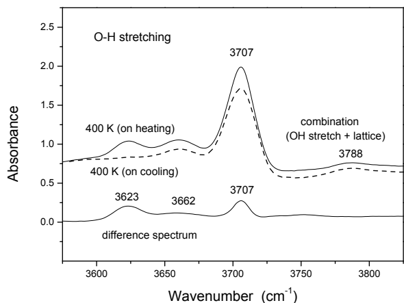
FIGURE 5. Difference spectrum between OH stretching bands recorded at 400 K before and after heating to 1000 K. The difference spectrum reveals the 3623 cm -1 band disappeared due to heating, whereas partial dehydroxylation occurred for the main Mg 3 -OH species that produced the stretching band near 3707 cm -1 .
