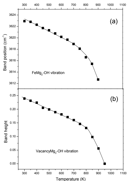
FIGURE 6. (a) Band frequency and (b) area of the 3623 cm -1 OH stretching vibration as a function of temperature.
