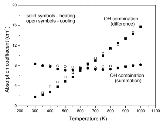
FIGURE 9. Absorption coefficients (calculated by absorbance over thickness in centimeters) for the combination band (summation) near 3402 \text{cm}^{-1} and combination (difference) near 3102 \text{cm}^{-1} . The solid symbols indicate data from heating whereas the open symbols are data on cooling. The results indicate that different types of combination bands of OH can have very different changes in band heights on heating.
