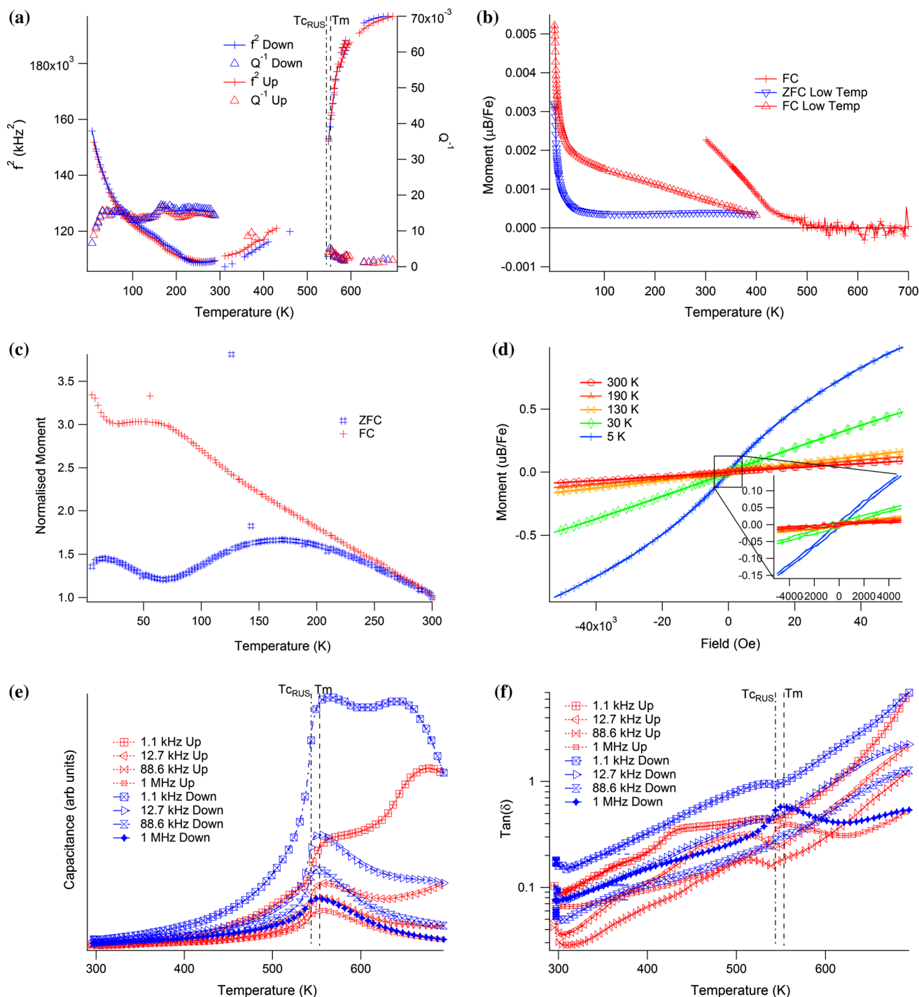
Figure 5 PZTFN4. a RUS analysed data showing f^2 and Q^{-1} , with scaling applied to match f^2 values at room temperature. b SQUID 2 temperature dependence of the magnetic moment between \sim 2 and 700 K measured under an applied field of 0.01 T. Triangular markers (one marker displayed per four data points) show ZFC and FC data below room temperature; crosses (one marker displayed per two data points) show ZFC data above room temperature and FC data for the full temperature range. c SQUID
