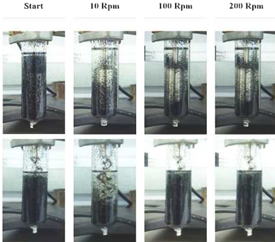
Fig. 7. Images of the distribution of particles in the viscometer using the f100 fluid for the SC4-27 spindle (top) and DHI (bottom) at the start of the test and after 10 minutes for various rotational speeds.
