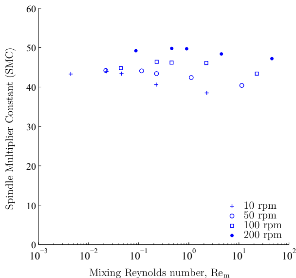
Fig. 11. Plot of the Spindle Multiplier Constant (SMC) against mixing Reynolds number for the DHI impellor.
