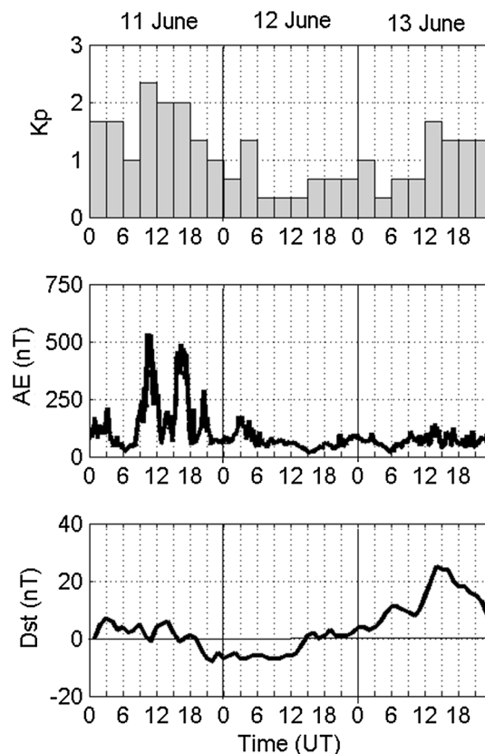
Fig. 1 Variation in the 3 hourly Kp (top), 1 min AE (middle) and 1 h Dst (bottom) indices during June 11–13, 2014
