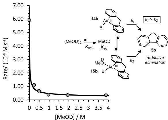
Figure 3. Effect of [\text{MeOD}] on the pseudo zero-order rate of catalyst turnover, k[\text{Au}] = (k_1[\mathbf{14b}] + k_2[\mathbf{15b}]) ; [\text{Au}] = 0.001 \text{ M} , 27 °C. Circles: experimental data. Solid line: simulation based on catalytic rate law (see SI) for scheme shown, with k_1/k_2 \geq 17 . Methanol is extensively dimerized in \text{CHCl}_3 ; 31 For x = 0 , trifluoroethanol (0.27 M) replaces MeOD.
