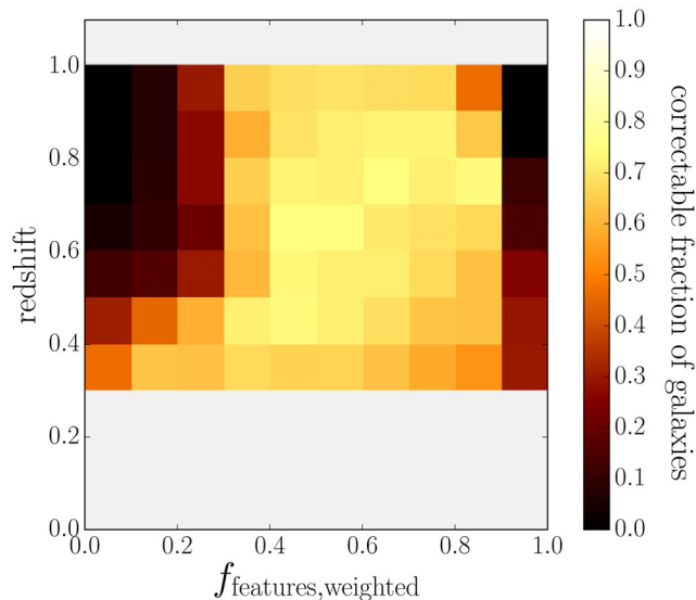
Figure 11. Histogram showing the fraction of galaxies that have a finite correction for the debiased vote fractions f_{\text{features, debiased}} as a function of f_{\text{features, weighted}} and redshift. The parameter space for corrections is limited to 0.3 \leq z \leq 1.0 due to the sampling of the parent SDSS galaxies and detectability in the FERENGI images.
