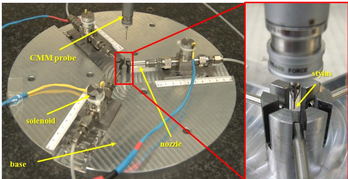
Figure 18 A prototype device for in situ cleaning of μCMM stylus tips using CO 2 snow [11]
