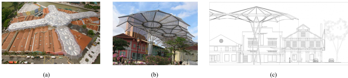
Fig.5. (a & b) Aerial and street view of the ETFE structure at Clark Quay; (c) Clarke Quay ETFE structure at 15m above ground (source: Archinet)
