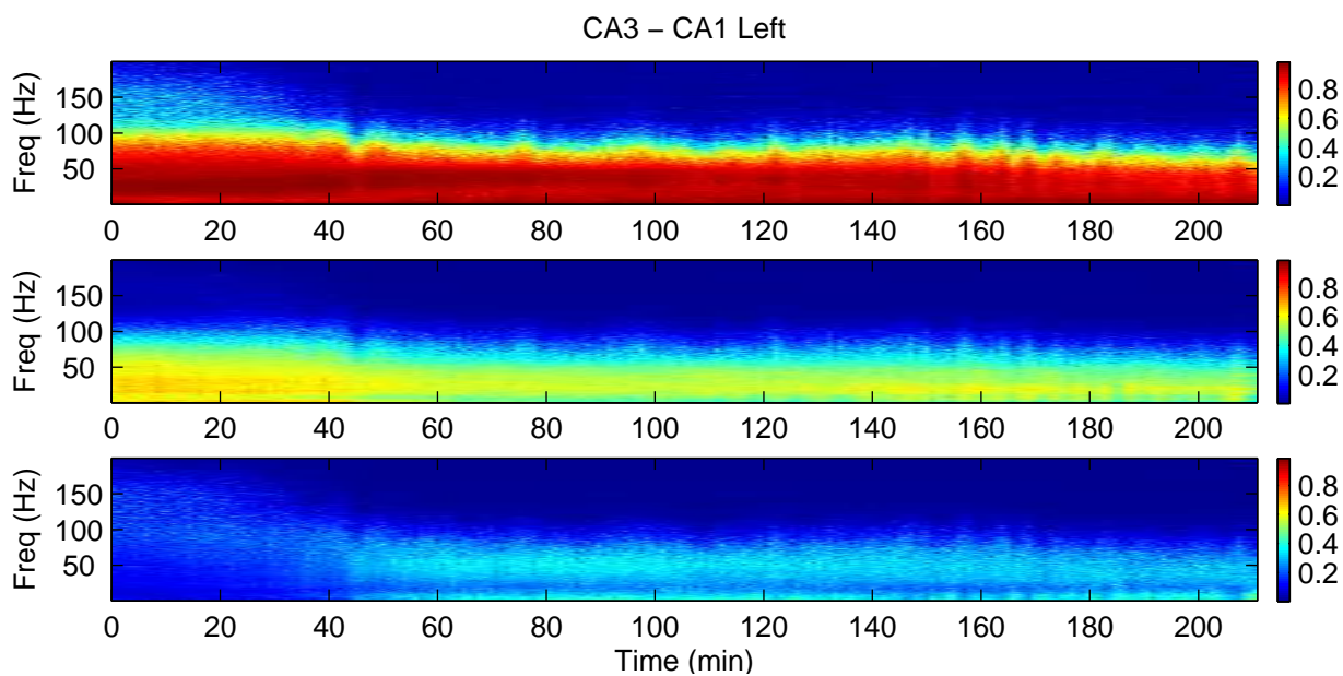
Figure 5: Bivariate directionality analysis of LFP recordings from CA3 and CA1 in left hippocampus in an anaesthetised rat. Kainic acid was injected locally into the left hippocampus at 30 minutes. The plots show the estimated coherence (top) and forward (CA3→CA1, middle) and reverse (CA1→CA3, bottom) components, with CA3 as the reference. Analysis was undertaken by splitting the complete record in to non-overlapping blocks of duration approximately 1 minute. Scale bars on the right indicate the strength of coherence (top) and directional (middle, bottom) components, all to the same scale. The 95% significance level for the coherence estimate (top) is 0.0512, based on the assumption of uncorrelated signals.
