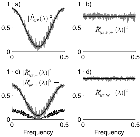
Figure 4: Conditional and unconditional directionality analyses of the relationship between four simulated processes, z_1 , z_2 (predictors) and x , y . a) Estimated ordinary coherence estimate between x and y (grey) compared with theoretical model (black). b) Estimated forward component of conditional coherence estimate with z_1 as predictor (grey) compared with theoretical model (black). c) Estimated forward (black) and reverse (grey) components of coherence estimate in panel a). The theoretical values are shown in grey and black for forward and reverse estimates, respectively. d) Estimated reverse component of conditional coherence estimate with z_2 as predictor (grey) compared with theoretical model (black). Plots are shown against fractional frequency where 0.5 corresponds to the Nyquist frequency. See text for parameters and further details.
