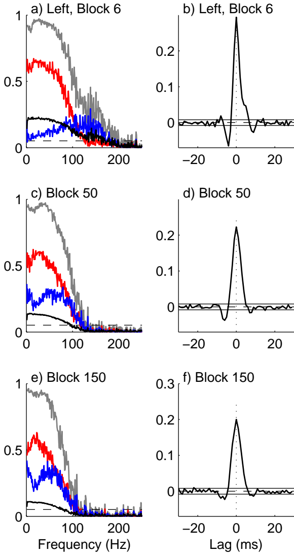
Figure 7: Directionality analysis for 1 minute blocks centred at 5.4 (block 6, top), 49 (block 50 centre) and 148 minutes (block 150 lower). Analysis is for CA3-CA1 interaction in left hemisphere (CA3-CA1 L), ipsilateral to local KA injection. Left column shows frequency domain analysis, with coherence (grey), forward component (red) reverse component (blue) and zero lag component (black). The dashed horizontal line is the estimated upper 95% confidence limit for the coherence based on the assumption of uncorrelated signals. Right column illustrates time domain analysis showing estimated correlation function, along with null value (dashed horizontal line) and upper and lower 95% confidence limits based on the assumption of uncorrelated signals. Further discussion in text.
