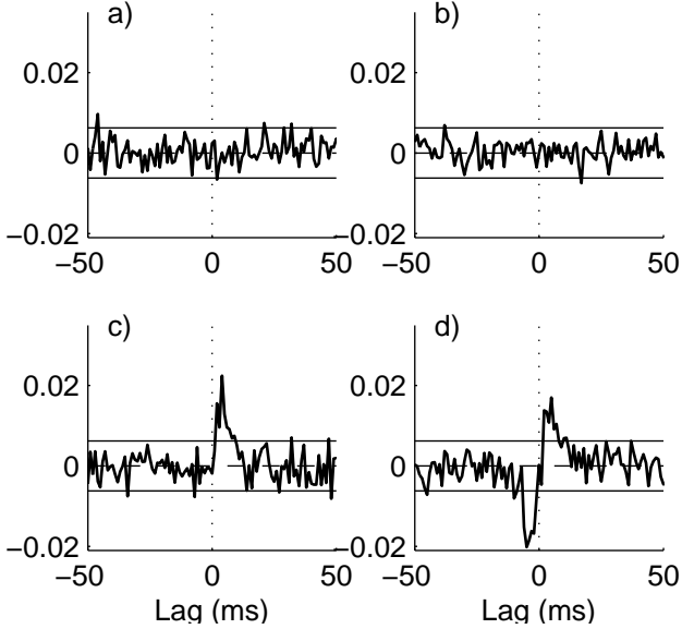
Figure 3: Conditional directionality analysis for interactions between neurons 2 and 3, conditioned on neuron 1. Configurations as shown in figure 1. Plots show the estimated conditional correlation function, \hat{\rho}_{32|1}(\tau) , along with null value (dashed horizontal line at zero) and upper and lower 95% confidence limits (solid horizontal lines) based on the assumption of uncorrelated processes. The lag ranges are the same for all panels, the vertical axes are the same as the corresponding plot in figure 2. A dotted vertical line at \tau = 0 is included for reference.
