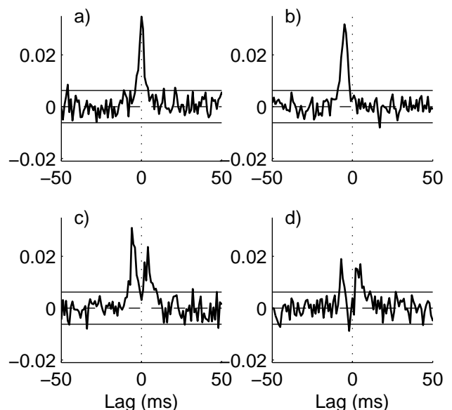
Figure 2: Bivariate directionality analysis for interactions between neurons 2 and 3. Configurations as shown in figure 1. Plots show the estimated correlation function, \hat{\rho}_{32}(\tau) , along with null value (dashed horizontal line at zero) and upper and lower 95% confidence limits (solid horizontal lines) based on the assumption of uncorrelated processes. The lag ranges are the same for all panels, a dotted vertical line at \tau = 0 is included for reference.
