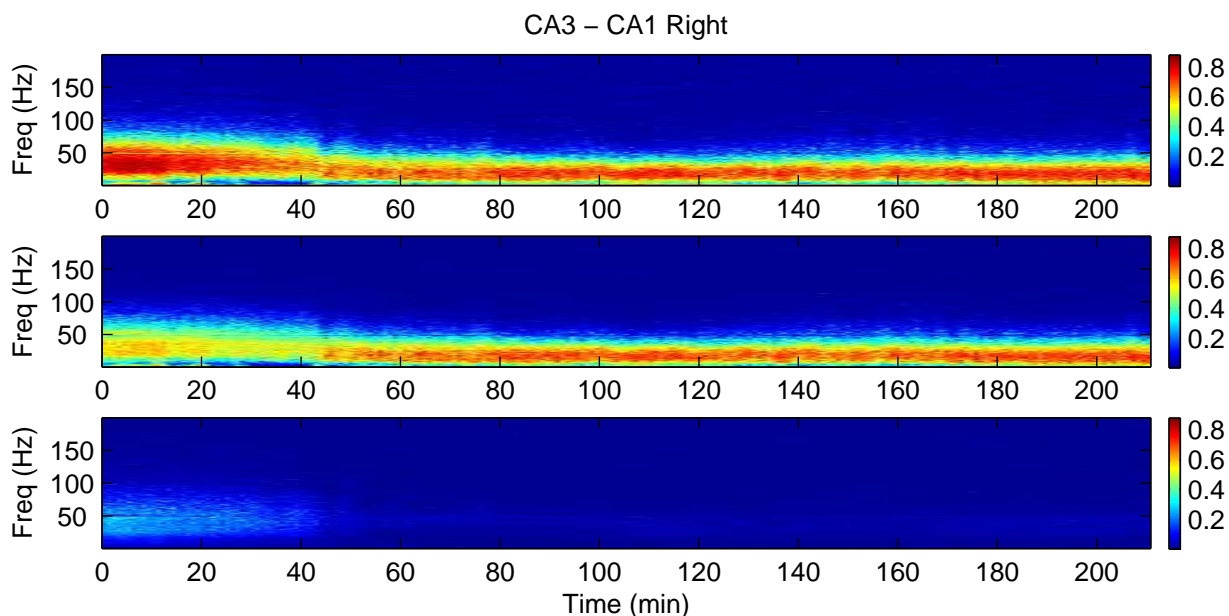
Figure 6: Bivariate directionality analysis of LFP recordings from CA3 and CA1 in right hippocampus in an anaesthetised rat. Kainic acid was injected into the left hippocampus after 30 minutes basal recording. The plots show the estimated coherence (top) and forward (middle) and reverse (bottom) components, with CA3 as the reference. Analysis used same parameters as for Left Hippocampus, see legend for Figure 5.
