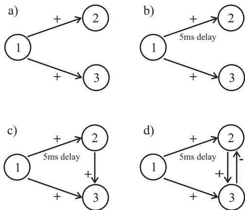
Figure 1: Network configuration for cortical network simulations. Excitatory connections are indicated: “+”, inhibitory connections are indicated: “-”. In configurations b) - d) the connection from 1 \rightarrow 2 has an additional synaptic delay of 5 ms.
