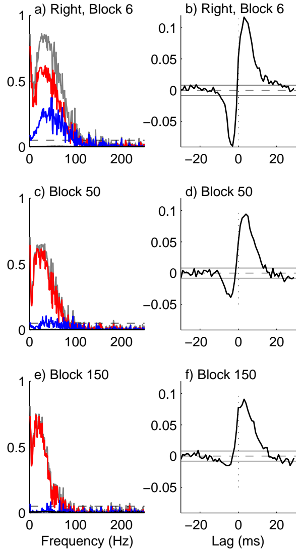
Figure 8: Directionality analysis for 1 minute blocks centred at 5.4 (block 6, top), 49 (block 50 centre) and 148 minutes (block 150 lower). Analysis is for hippocampal CA3-CA1 interaction in the right hemisphere (CA3-CA1 R), contralateral to local KA injection. Layout, format and confidence limits same as in figure 7. Further discussion in text.
