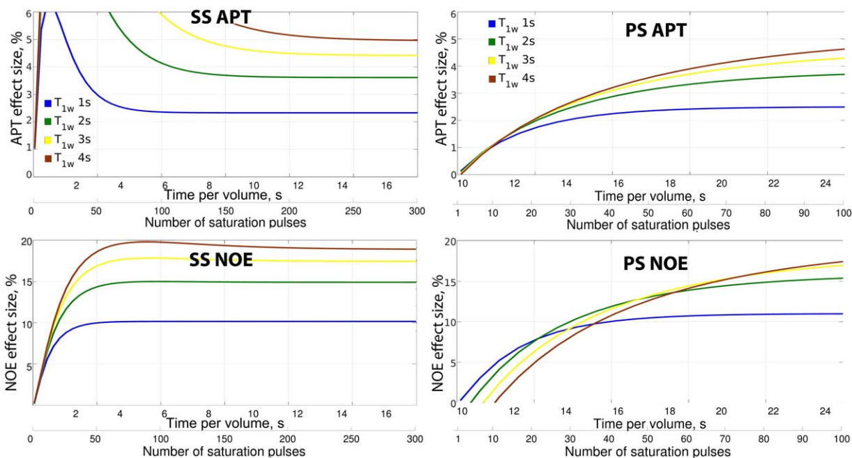
FIG. 3. Bloch-McConnell equations were used to simulate the APT and NOE contributions for SS and PS during the approach to SS, as a function of the number of saturation pulses (also recalculated as time-per-volume or dynamic scan time on the second axis) at a B_1 of 1 \mu\text{T} and various water- T_1 relaxation times. The frequency offsets used were 3.5 ppm and -3.5 ppm for APT and NOE, respectively.
