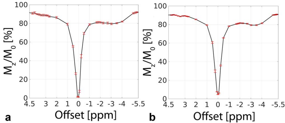
FIG. 6. Representative Z-spectra from a healthy volunteer for SS scheme (a) and PS scheme (b) acquired at an actual B_1 of 0.7 \mu\text{T} (ROI 1 in the Figure 2).
