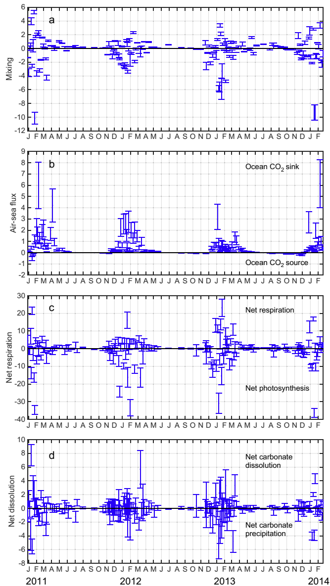
Fig. 6. Calculated rates of processes affecting DIC in the surface water of Ryder Bay, expressed in \mu\text{mol DIC kg}^{-1} \text{d}^{-1} . (a) Mixing, (b) air–sea \text{CO}_2 flux, (c) net respiration and (d) net dissolution. Error bars represent approximate 95% confidence from Monte Carlo analysis.
