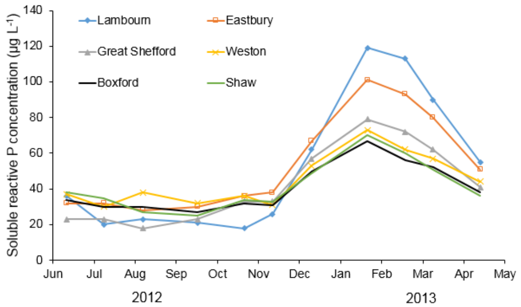
Fig. 7. Soluble reactive phosphorus concentrations at multiple points along the River Lambourn 2012-2013. Locations of sampling points are shown in Figure 1.
