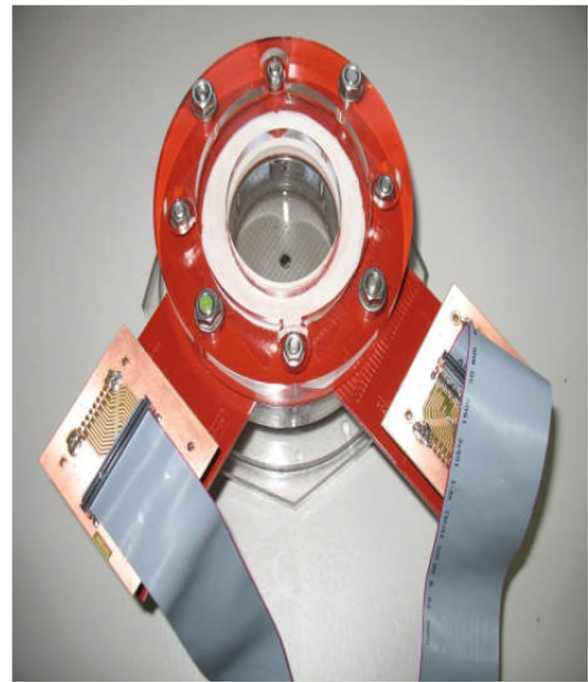
Fig. 2. WMS sensor.
