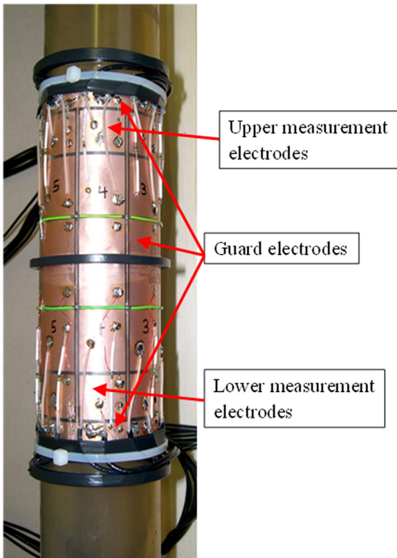
Fig. 1. ECT sensor.
