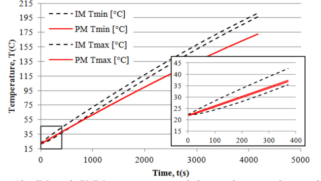
Fig. 13. IM and PMM temperature variation under normal operating conditions.
