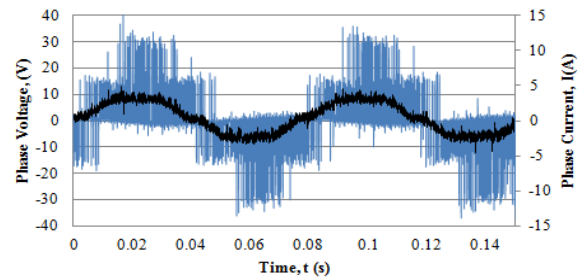
Fig. 17. Measured phase voltage and current of IM under no load operation at 180 rpm.
