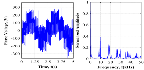
Fig. 18. Measured phase voltage and respective harmonic content of IM at 6000rpm.
