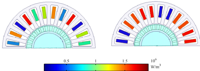
Fig. 9. Power loss density distribution under normal (left) and extreme (right) operating conditions.
