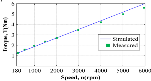
Fig. 22. Comparison of simulated and measured torque-speed characteristic.
