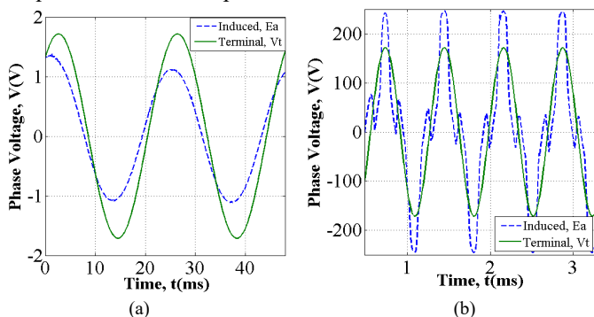
Fig. 10. Induced and terminal phase voltage under normal (a) and extreme (b) conditions.
