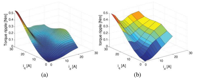
Fig. 23. Prototype 3C: torque ripple surface over the i_d , i_q plane, according to FEA (a) and measurements (b).
