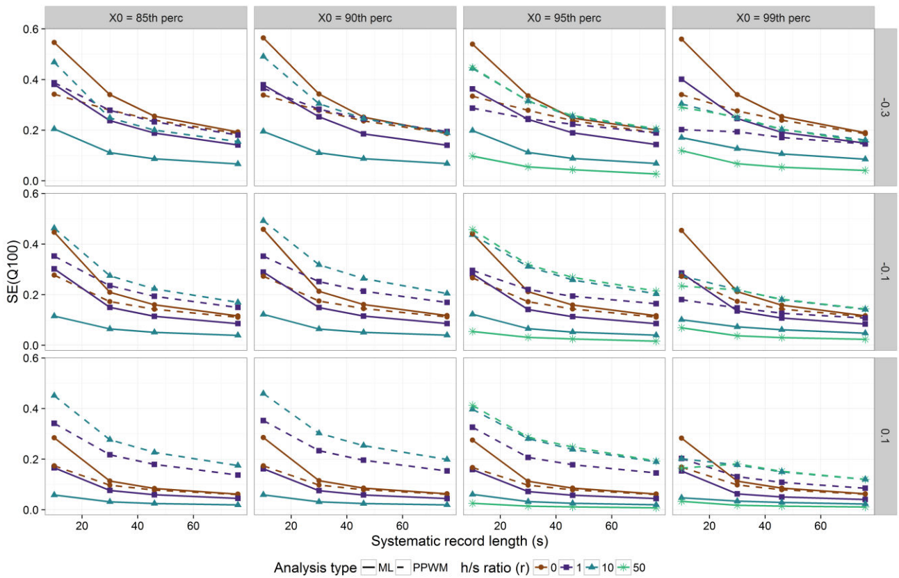
Figure 8. As Figure 6, showing the SE for the \log(Q_{100}) .
