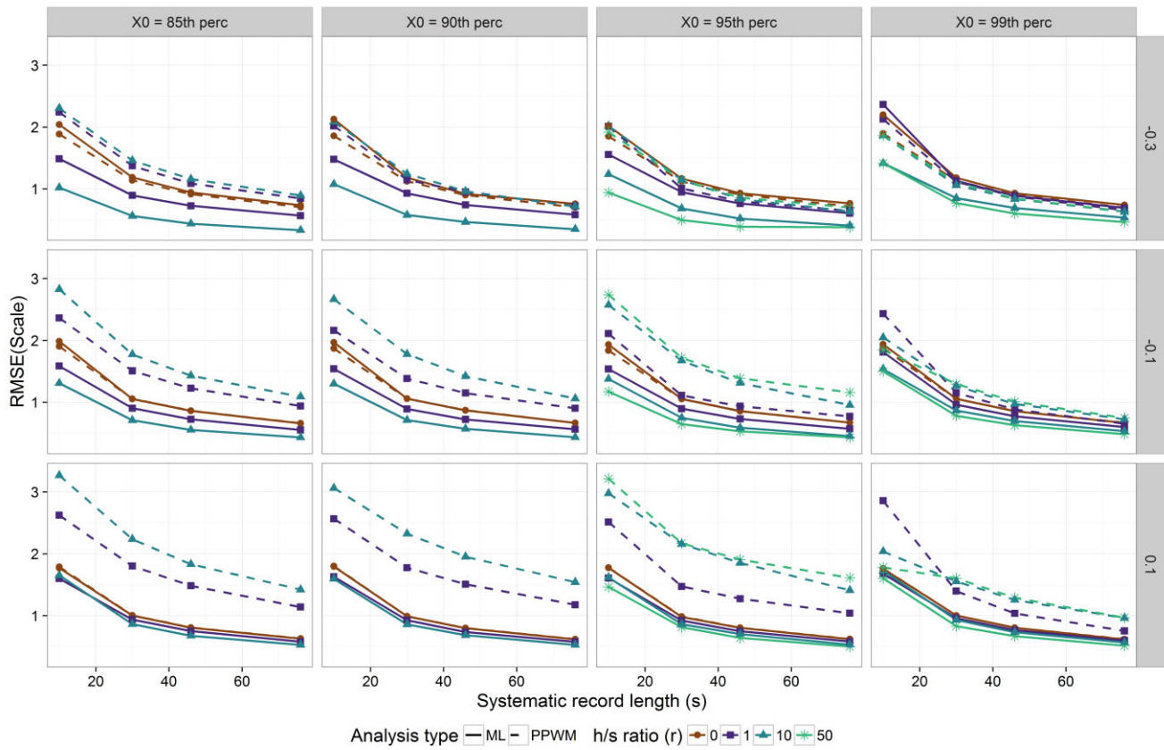
Figure 2. RMSE for the scale parameter as a function of the systematic record length, for selected historical record lengths for all estimation methods (ML: continuous line; PPWM: dashed line). Each panel shows different X_0 and shape parameter combination. Parent distributions L-CV is 0.2
