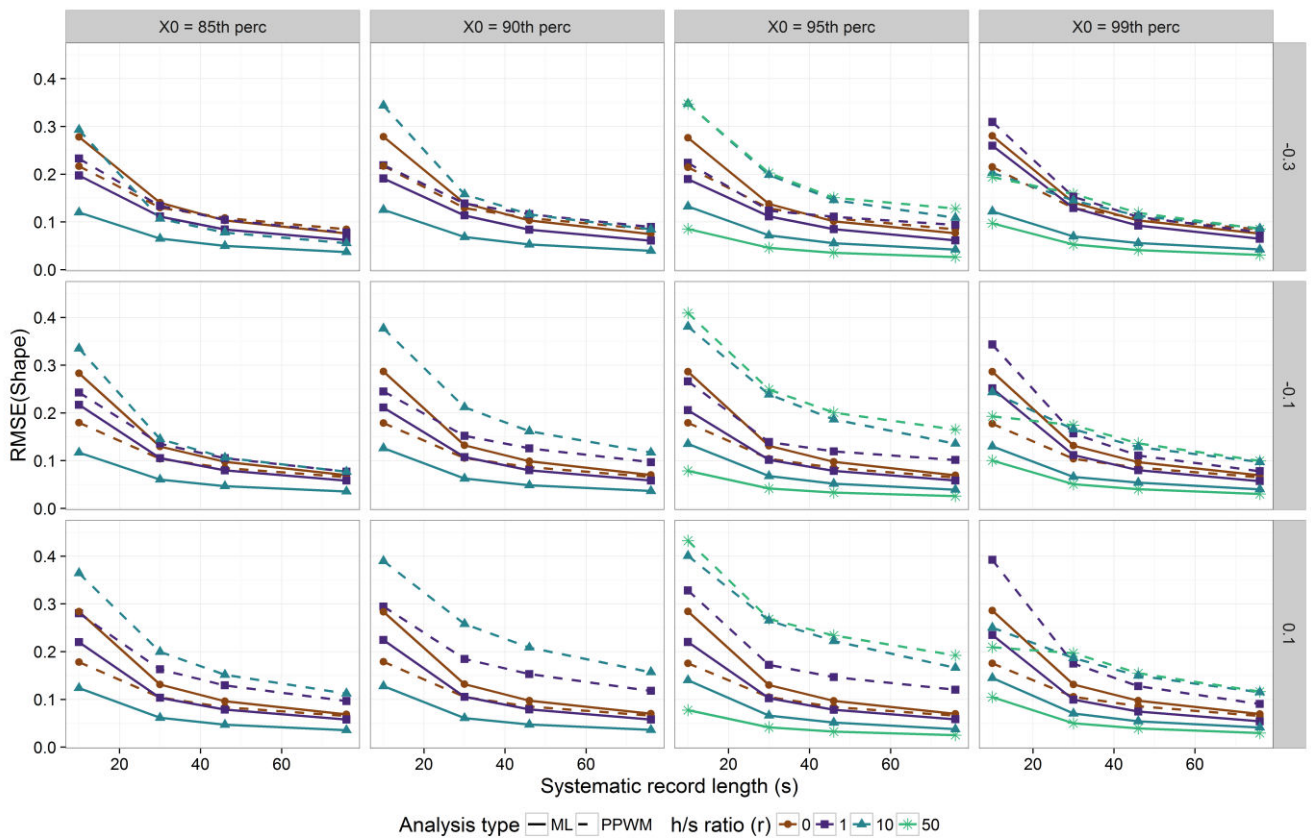
Figure 3. As Figure 2, RMSE for the shape parameter.
