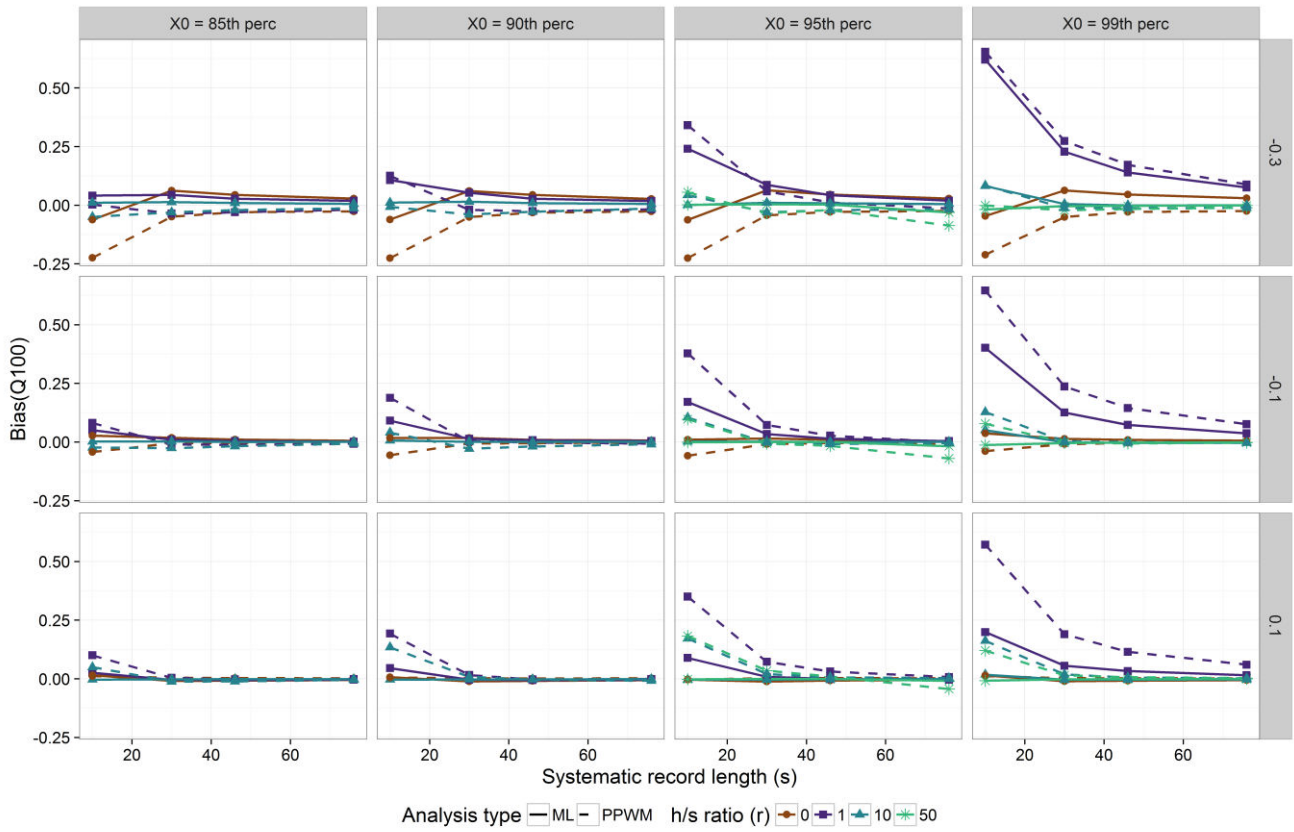
Figure 7. As Figure 6, showing the Bias for the \log(Q_{100}) .
