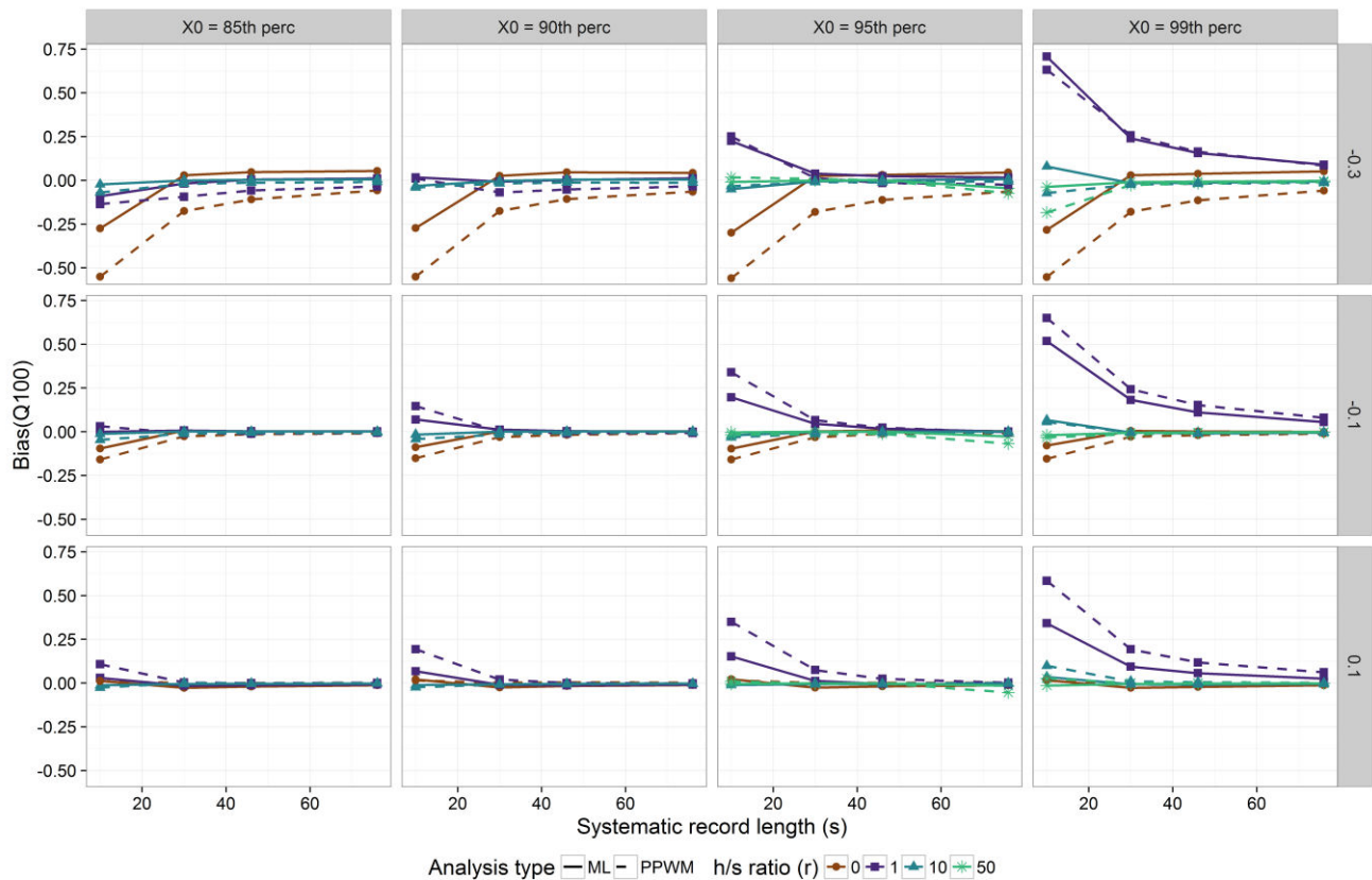
Figure 10. As Figure 9, showing the Bias for the \log(Q_{100}) .
