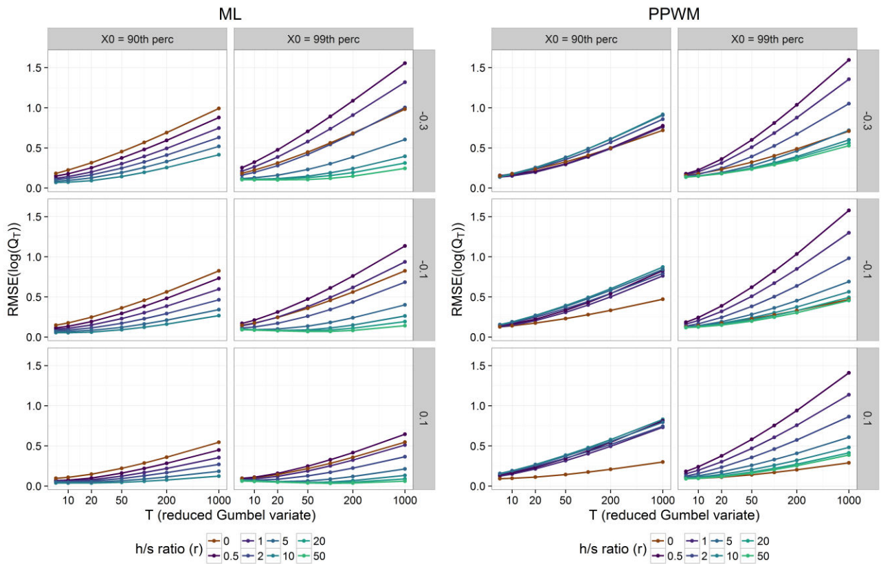
Figure 12. RMSE for Standard Error for \log(Q_T) as a function of T (on a Gumbel scale). Systematic sample size: 10. Each panel shows selected combinations of X_0 and shape parameter. Left panel: ML results; right panel: PPWM results Parent distributions L-CV is 0.2.
