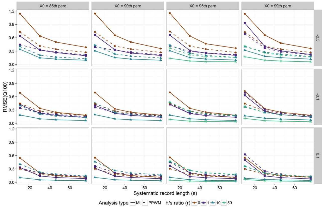
Figure 9. RMSE for the \log(Q_{100}) as a function of the systematic record length, for selected historical record lengths for all estimation methods (ML: continuous line; PPWM: dashed line). Each panel shows different X_0 and shape parameter combination. Parent distributions L-CV is 0.9.
