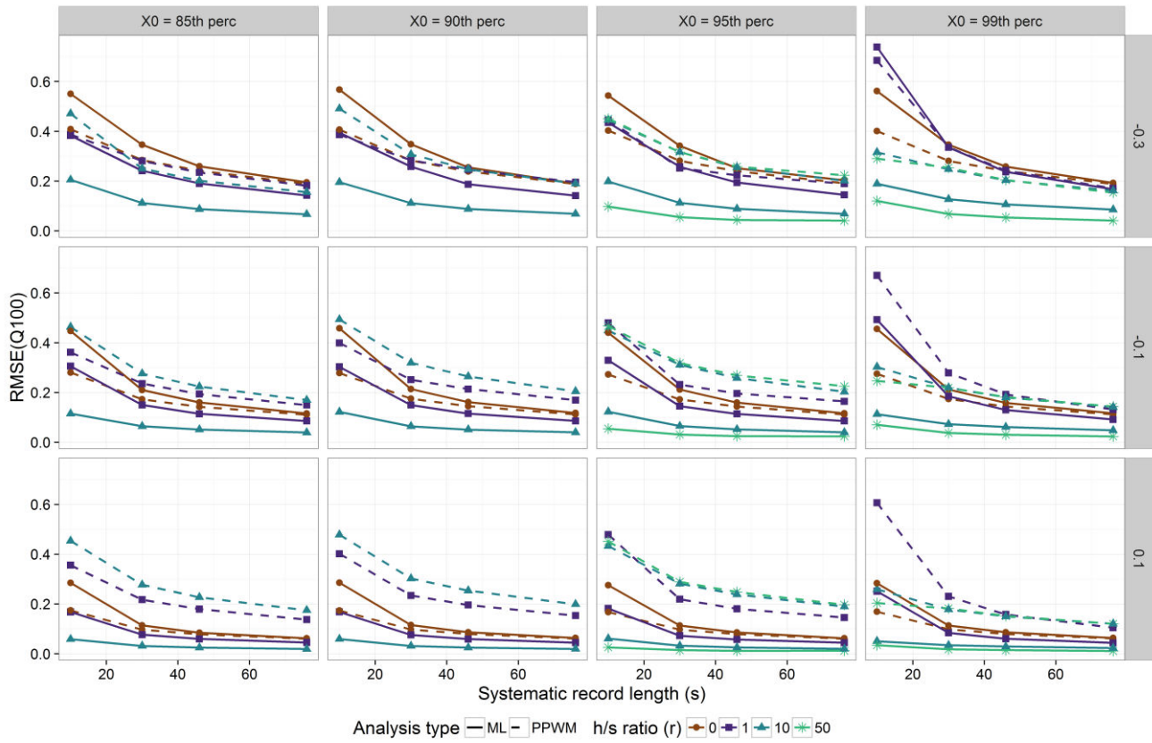
Figure 6. RMSE for the \log(Q_{100}) as a function of the systematic record length, for selected historical record lengths for all estimation methods (ML: continuous line; PPWM: dashed line). Each panel shows different X_0 and shape parameter combination. Parent distributions L-CV is 0.2.
