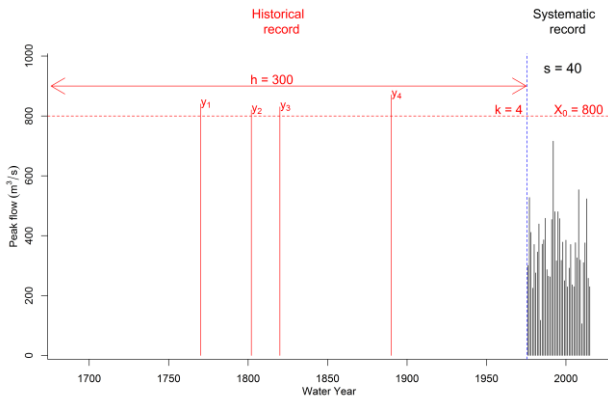
Figure 1. Historical data example, showing a total of k=4 historical events (red bars) above the perception threshold X_0 (dashed red line), recorded across the h=300 year long historical period. The s=40 years long systematic record of gauged peak flows is also shown (black bars).
