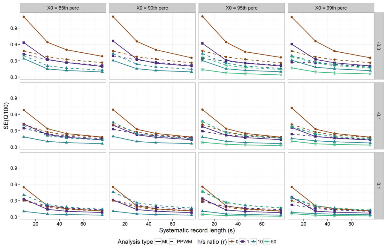
Figure 11. As Figure 9, showing the SE for the \log(Q_{100}) .
