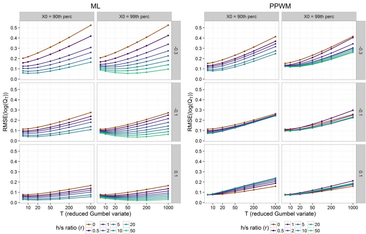
Figure 15. As Figure 14; sample size: 76.
