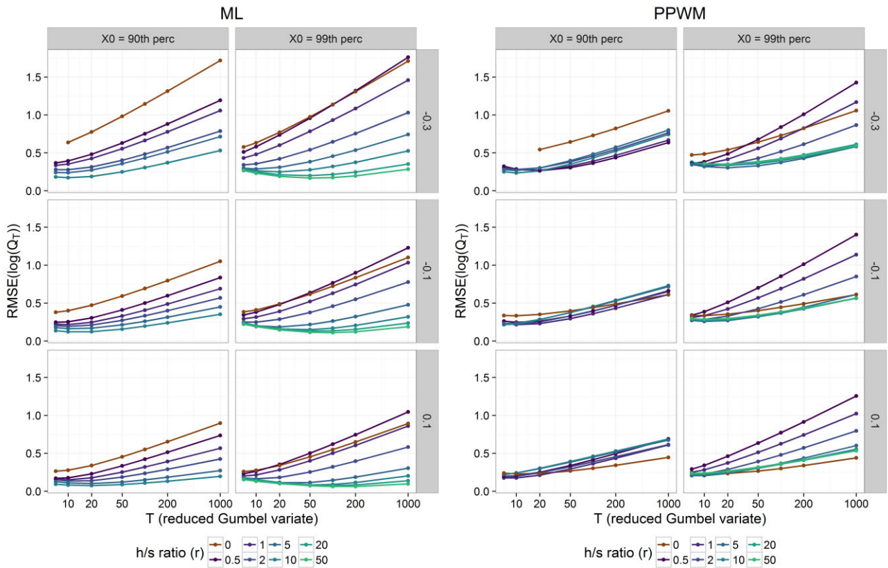
Figure 14. RMSE for Standard Error for \log(Q_T) as a function of T (on a Gumbel scale). Systematic sample size: 10. Each panel shows selected combinations of X_0 and shape parameter. Left panel: ML results; right panel: PPWM results Parent distributions L-CV is 0.9
