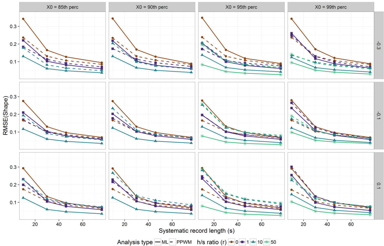
Figure 5. As Figure 4, RMSE for the shape parameter.
