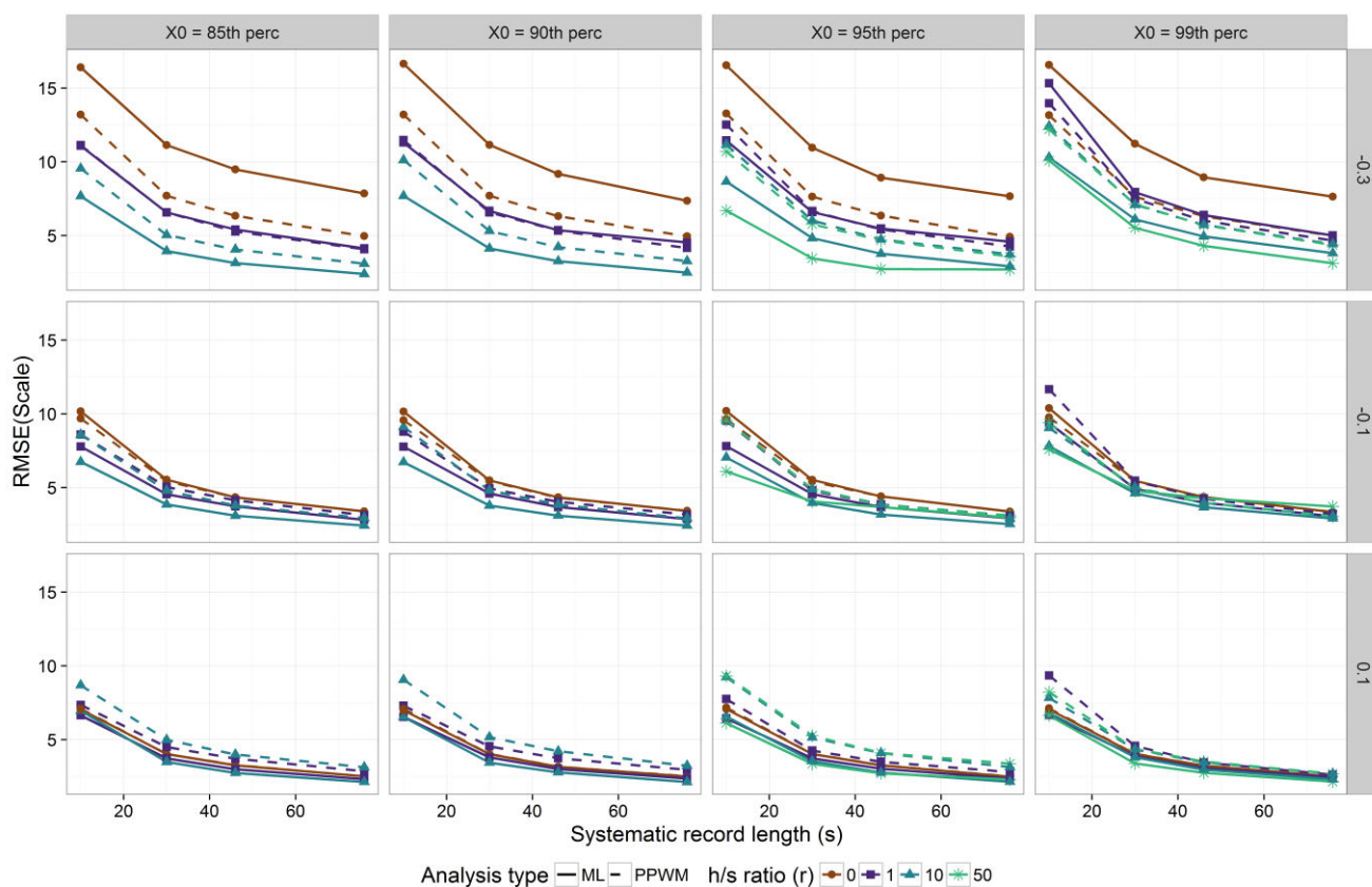
Figure 4. RMSE for the scale parameter as a function of the systematic record length, for selected historical record lengths for all estimation methods (ML: continuous line; PPWM: dashed line). Each panel shows different X_0 and shape parameter combination. Parent distributions L-CV is 0.9.
