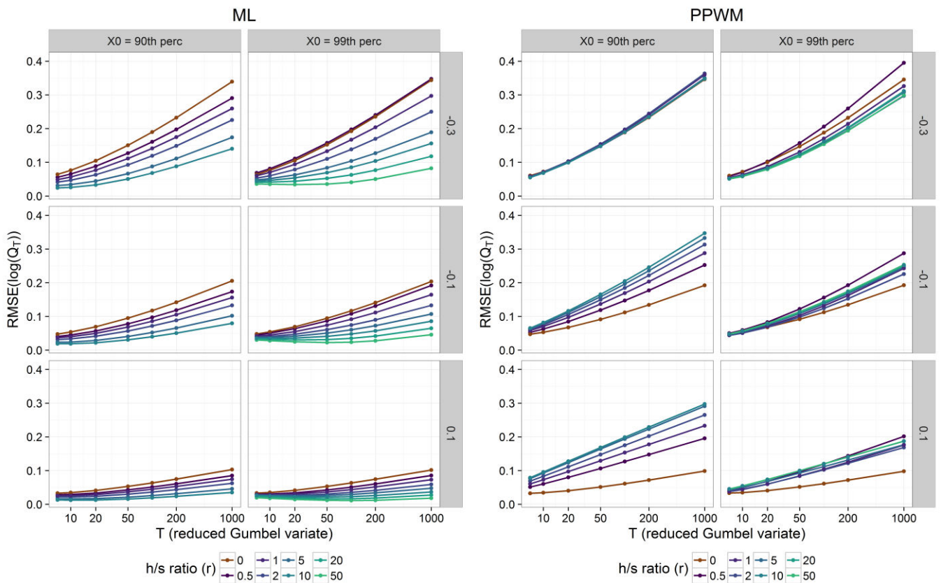
Figure 13. As Figure 12; sample size: 76.
