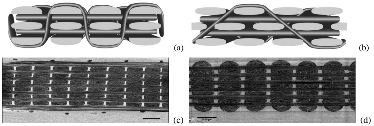
Fig. 1 Cross-sections of 3D woven fabrics; geometrical models of orthogonal (a) and angle-interlock (b) fabrics, normal to weft direction; \mu -CT scans [5] of an orthogonal fabric, normal to warp direction (c) and normal to weft direction (d) .
