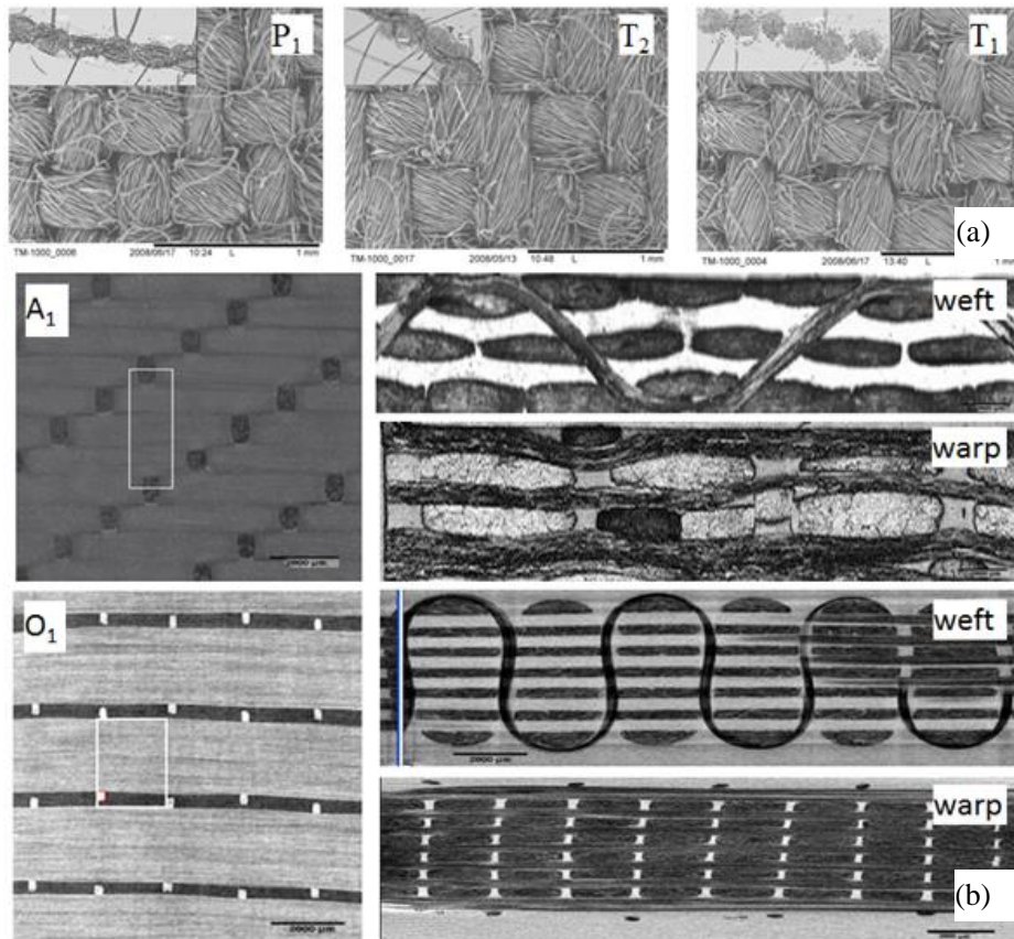
Fig. 5 (a) Top views and cross-sections of woven fabrics P 1 , T 1 , T 2 ; (b) top views and cross-sections normal to warp and weft directions of fabrics A 1 and O 1
