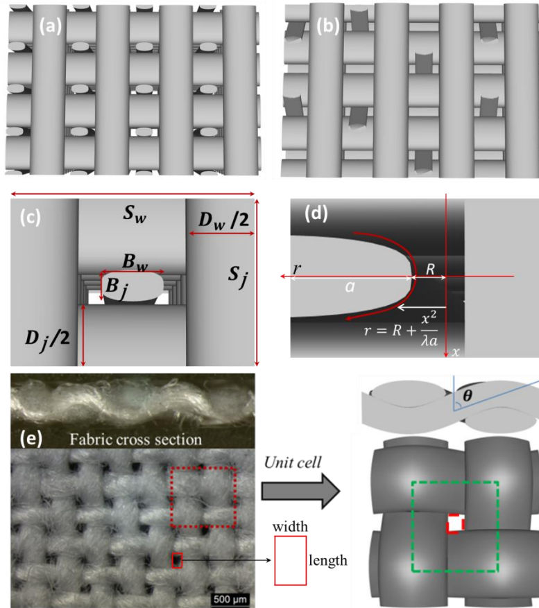
Fig. 3 Top view of orthogonal (a) and angle-interlock (b) fabrics; top view of a unit-cell of orthogonal weave (c) and side view normal to warp direction (d) with dimensions; (e) left: top and side views of a plain weave fabric; (e) right: fabric unit-cell where the red frame indicates the inter-yarn gap, and the green frame indicates the yarn area; \theta is the yarn crimp angle.
