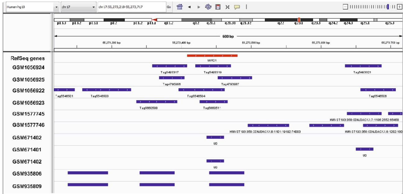
Supplementary Figure S1: The NCBI-GEO database ( http://www.ncbi.nlm.nih.gov/geo/ ) was searched for STAT5 chromatin-immunoprecipitation (ChIP) coupled with next generation sequencing (ChIPseq) or array (ChIP-chip). Peaks (in BED) format were converted to HG18 coordinates using the UCSC-Liftover tool where necessary and visualized using the Integrated Genome Viewer. ( http://www.ncbi.nlm.nih.gov/geo/ ). STAT5B occupancy of the miR21 locus (indicated in red) is and IL2 stimulated (GSM1577746) pre-activated CD8 + T cells; control (GSM671401) evident in human conventional T cells (GSM1056924, GSM1056925), human T regulatory cells (GSM056922, GSM1056923); control (GSM1577745) and IL2 stimulated (GSM671402) Th1 T cells and human erythroleukemic cells (GSM935806). Interestingly, STAT5B coincides with p53 at the miR21 locus in human leukemic cells (GSM935809).
