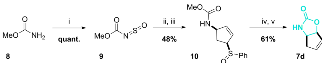
Scheme 3. Synthesis of 7d via an allylic sulfoxide rearrangement. i - \text{SOCl}_2 , \text{Py} , \text{Et}_2\text{O} , RT, 3 h. ii - cyclopentadiene, \text{PhH} , RT, 24 h. iii - \text{PhMgBr} , \text{THF} , RT, 20 min. iv - \text{P}(\text{OMe})_3 , \text{EtOH} , \Delta , 36 h. v - \text{KOH} , \text{MeOH} , RT, 24 h.
