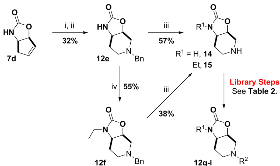
Scheme 5. Alternative route to the synthesis of library compounds ( 12 ) from 7d . i - O_3 , MeOH, -78\text{ }^\circ\text{C} . ii - \text{NaBH}_3\text{CN} , \text{BnNH}_2 , 0\text{ }^\circ\text{C} . iii - \text{H}_2 (1 atm.), Pd/C, HCl, MeOH, RT, 18 h. iv - n\text{BuLi} , EtI, THF, -78\text{ }^\circ\text{C} .
