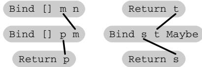
Figure 1. Graph produced by the separation algorithm from the example.
