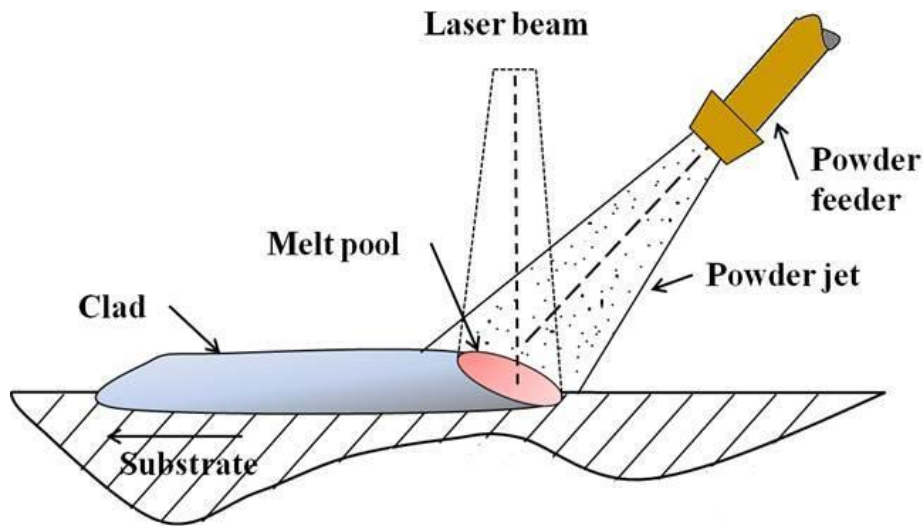
Fig. 1 Schematic of the powder laser cladding process.
