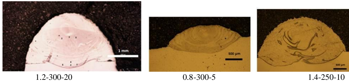
Fig. 4 Optical images of cross sections of laser cladding tracks for the cladding parameters indicated.
