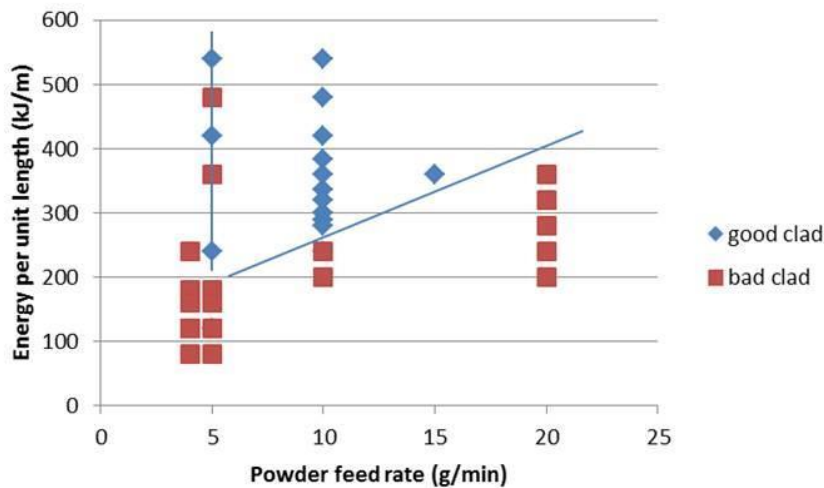
Fig. 5 Variation of clad quality across the parameter space used, the two lines outline the process window.
