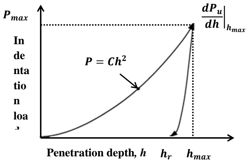
Fig. 1. A typical loading and unloading curve from an indentation test [1],
