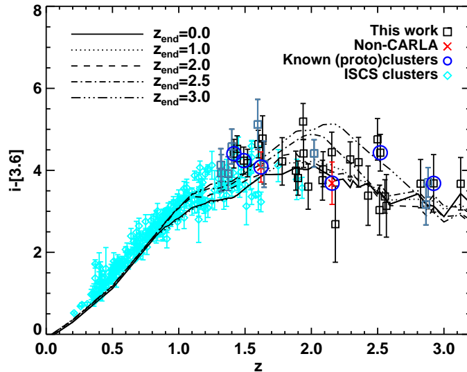
Figure 2.11: The same as Figure 2.10, but the different lines here correspond to different cut-offs in star formation, i.e. star formation is allowed to continue down to z_{end} , following the cosmic star formation rate density, and then terminated. The choice of z_{end} has little effect on the expected colours, suggesting that the cosmic star formation rate density itself is sufficient, requiring no cut-off.
