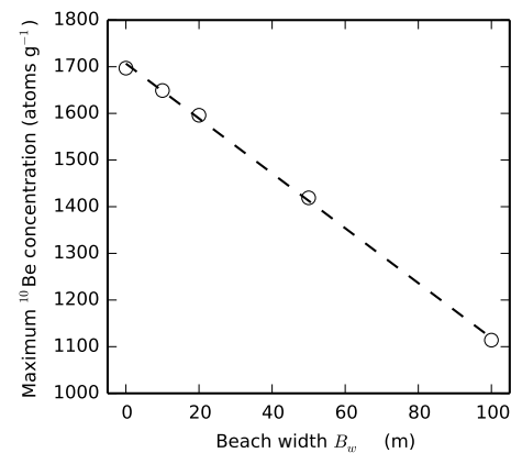
Figure 9. Reduction in the magnitude of peak concentration of ^{10}\text{Be} with increasing beach width. Black symbols show the peak concentrations taken from Fig. 8. The relationship is approximately linear as shown by the dashed line fit by least squares regression. Note that quite extreme beach cover B_w \geq 50 m is required to significantly ( \geq 15\% ) reduce platform ^{10}\text{Be} concentrations.
