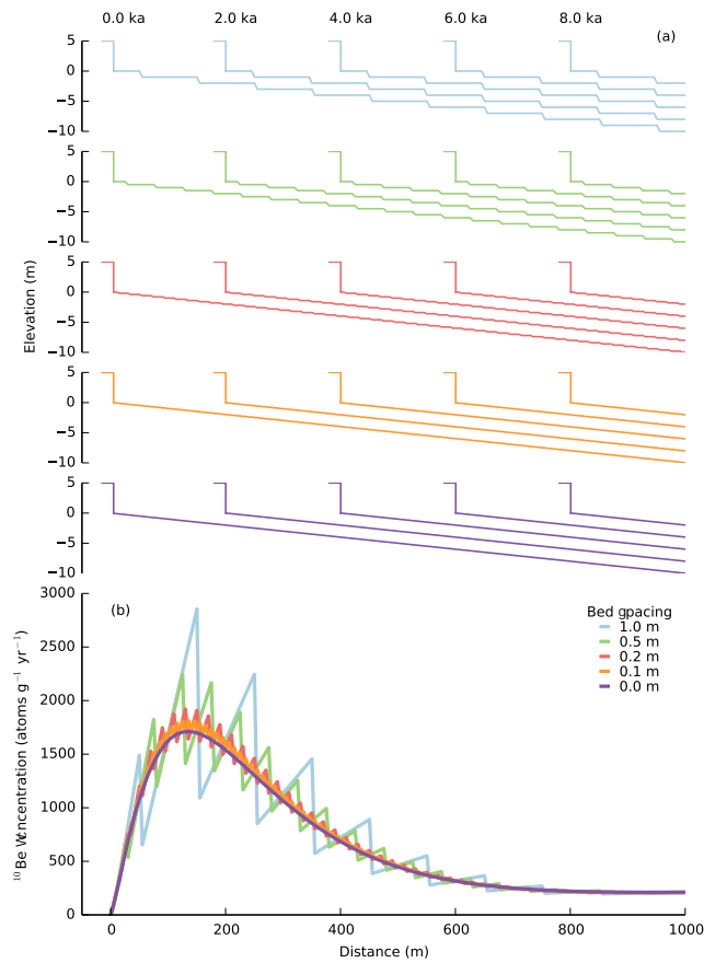
Figure 7. (a) Evolution of stepped shore platform profiles over 10 kyr for step sizes (bedding thickness) up to 1 m. (b) Corresponding distribution of ^{10}\text{Be} as a function of step size. Large steps due to block removal processes result in a saw-toothed distribution superimposed on the expected humped distribution. Variability in the platform surface concentration increases with step size.
