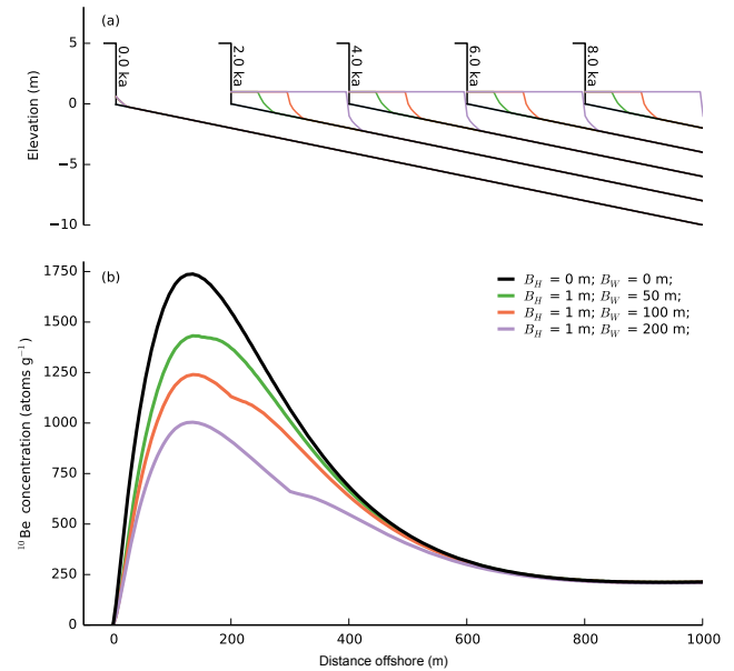
Figure 11. (a) Evolution of shore platform profiles over 10 kyr with variable beach cover in the near-shore zone described by a Bruun profile (Eq. 6). Beach width reduces to B_w = 0 m during the last 1000 years of the model runs. (b) Corresponding distribution of ^{10}\text{Be} for the case with no beach cover and thinning beaches during the last 100 years. The presence of beaches that disappeared over the last 1000 years would result in lower concentrations of ^{10}\text{Be} in the platform surface.
