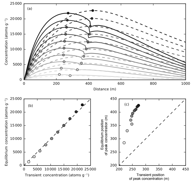
Figure 13. Comparison of transient simulations from Fig. 12 to predictions assuming steady-state profile retreat. Steady-state models are run with the constant retreat rate taken as the median values in the transient simulations (Fig. 12). Colour coding corresponds to the median retreat rates reported in Fig. 12b and the instantaneous mean platform gradient for each profile in Fig. 12a. (a) Distribution of ^{10}\text{Be} concentration predictions. The magnitude of the hump is similar as shown in panel (b) , but the location of the peak in concentration is further offshore when steady-state retreat is assumed, as also shown in panel (c) .
