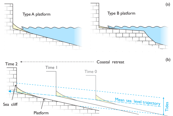
Figure 2. (a) Endmember types of shore platform as defined by Sunamura (1992). (b) Illustration of steady-state shore profile retreat subject to relative sea level rise.
