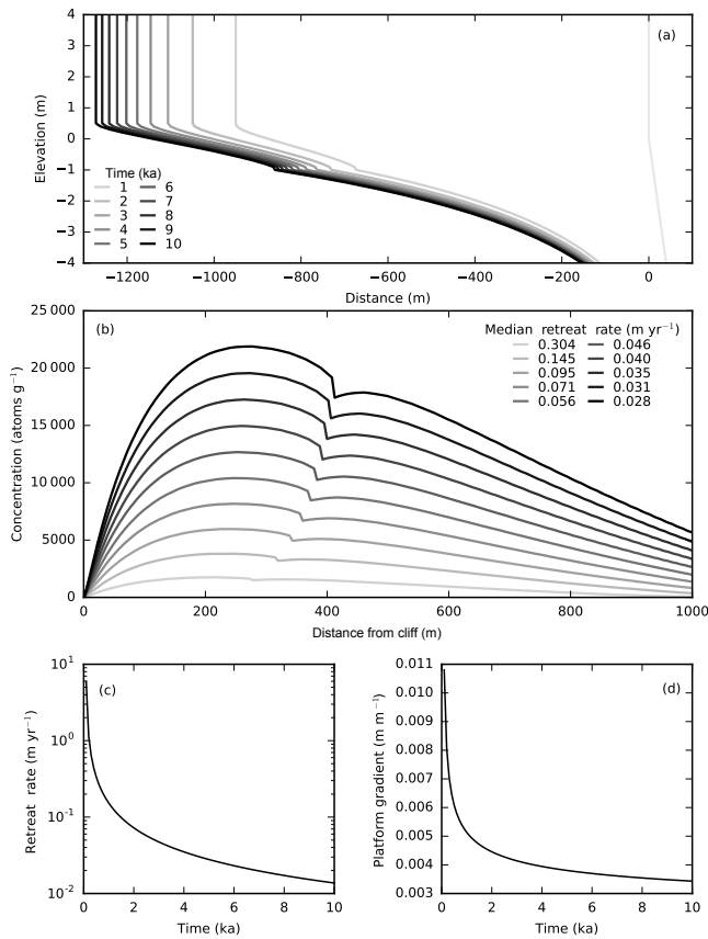
Figure 12. Transient simulations of shore profile evolution and ^{10}\text{Be} concentrations for the case with no sea level rise. (a) Evolution of shore platform profiles over 10 kyr driven by RoBoCoP (colour-coded in 1 kyr interval). (b) Corresponding ^{10}\text{Be} concentration predictions, normalized to the position of the cliff (colour coding also corresponds to the median retreat rates listed). Retreat rates are initially rapid and decline through time (c) and show a humped distribution, similar to steady-state model predictions. The magnitude of the hump increases through time as the length of exposure increases and cliff retreat rates and platform downwear rates decline, resulting in a decrease in platform gradient through time (d) .
