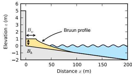
Figure 3. Example of beach model used in modelling 10 Be accumulation in a shore platform. Beach is defined by a beach width B_w and berm height B_h and a Bruun profile (Bruun, 1954) seaward of the defined beach width.
