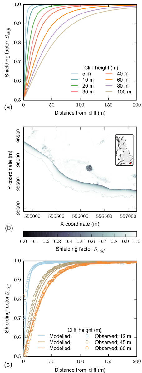
Figure 4. Topographic shielding due to sea cliff. (a) Analytical model for topographic shielding on a shore platform as a function of distance from cliff measured according to Eq. (11) for cliff heights ranging from 5 to 100 m. (b) Example map of the distribution of topographic shielding across a shore platform at Beachy Head, East Sussex, UK. (c) Comparison of Eq. (11) to values measured using distributed shielding routines (Codilean, 2006; Mudd et al., 2016).
