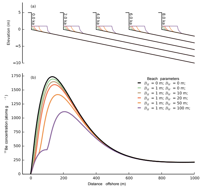
Figure 8. (a) Evolution of shore platform profiles over 10 kyr with constant beach cover in the near-shore zone described by a Bruun profile (Eq. 6). (b) Corresponding distribution of ^{10}\text{Be} as a function of beach width. Beach cover reduces the concentrations of ^{10}\text{Be} in the platform surface, and wider beaches result in lower ^{10}\text{Be} concentrations and cause the position of the peak in concentrations to be further out from the cliff. Note that quite extreme beach cover B_w \geq 50 m is required to significantly ( \geq 15\% ) reduce platform ^{10}\text{Be} concentrations.
