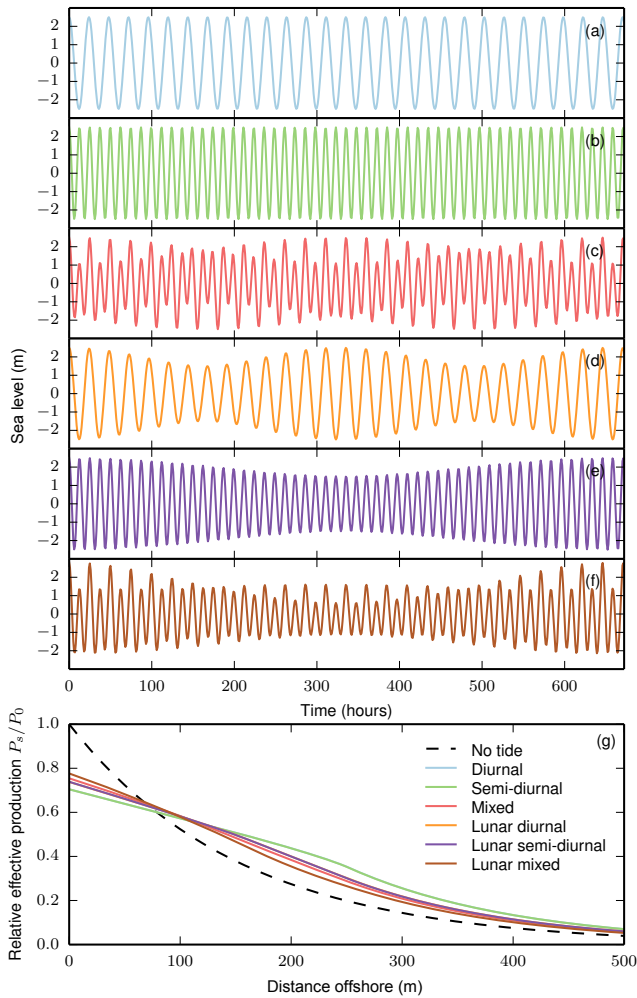
Figure 5. Influence of tidal regime on the distribution of 10 Be production across a shore platform. (a–f) Tidal water levels over a 28-day period for the hypothetical tidal regimes explored here (see Table 1). (g) Production rates relative to the case where there is no water shielding ( h_w = 0 ) as a function of distance offshore on a shore platform with gradient \alpha = 1/100 for the different tidal regimes plotted in panels (b–g).
