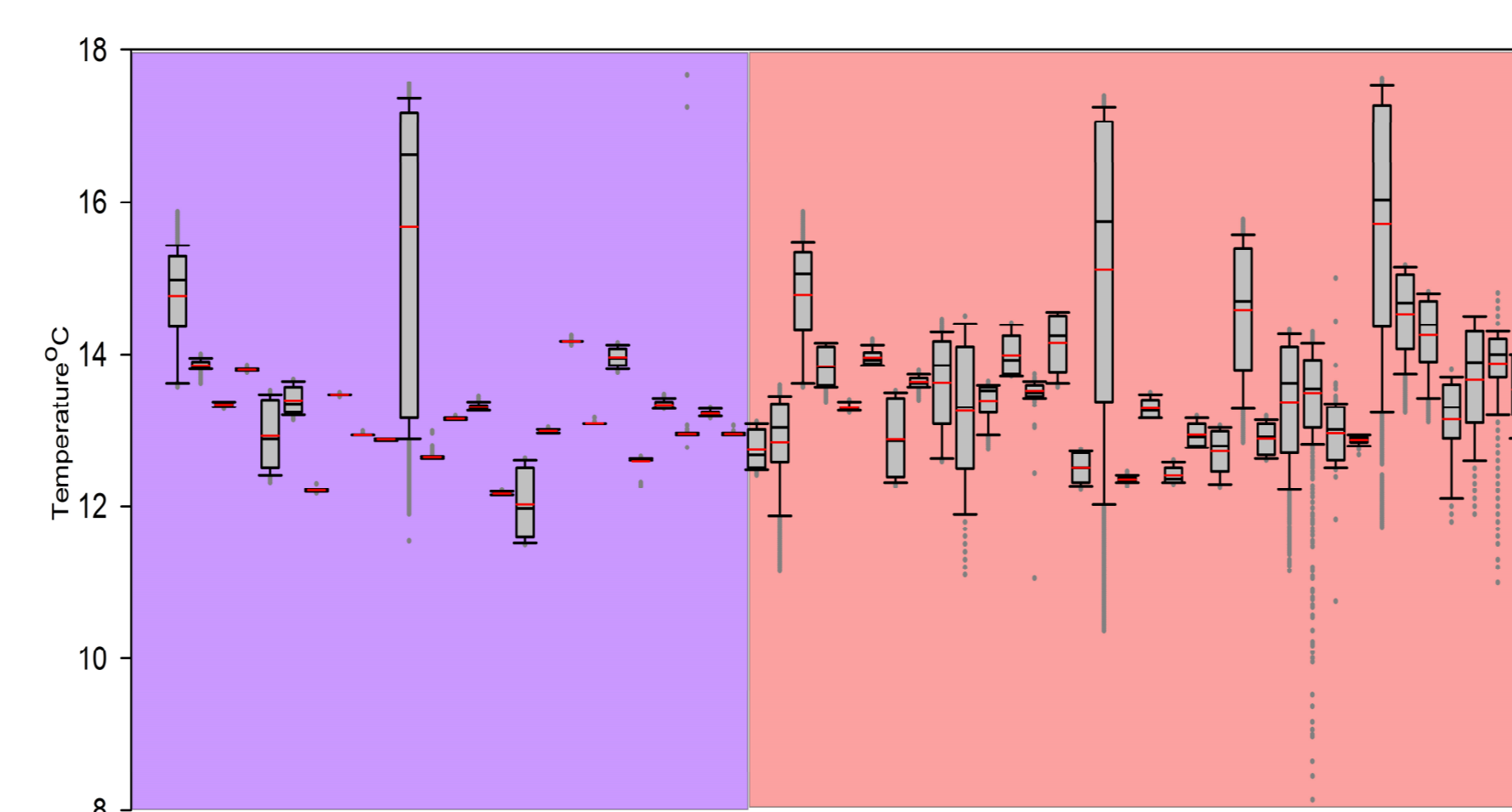
Fig. 4. Logger temperature variation during first 7 months (Jun15-Jan16). Purple - logger below the mean Zone of Seasonal Fluctuation (9.5mbgl), red - loggers within it
