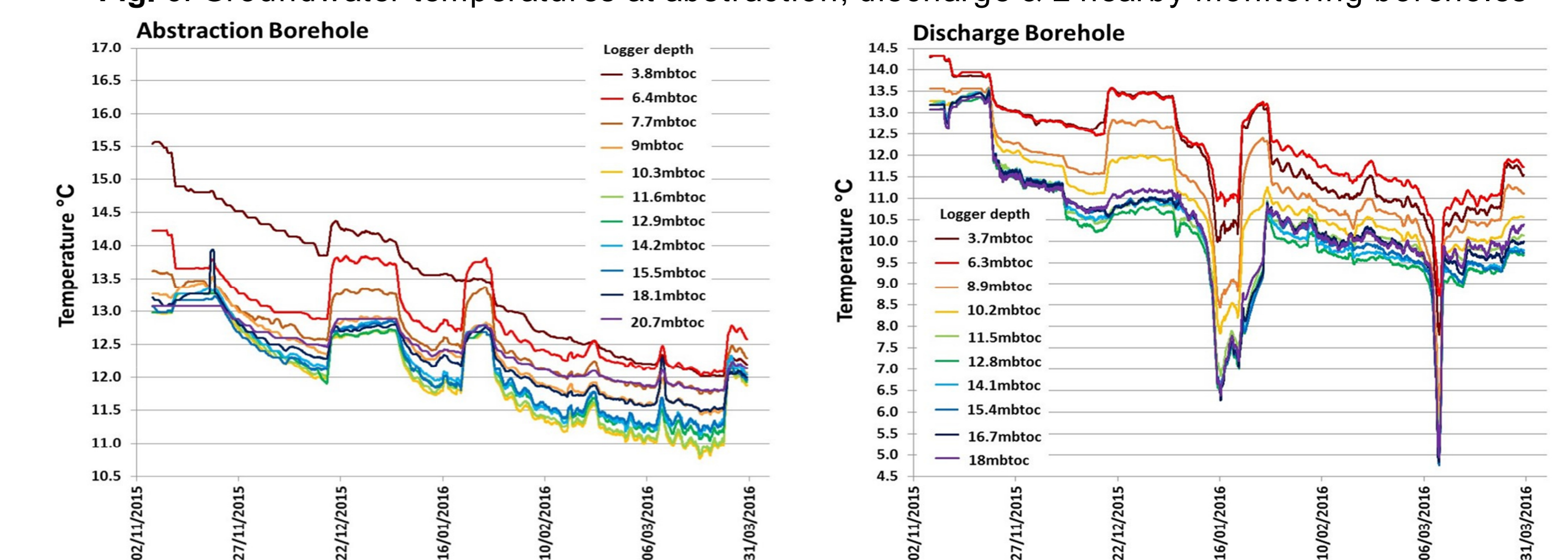
Fig. 7. Groundwater temperature at various depths in the abstraction & discharge boreholes
