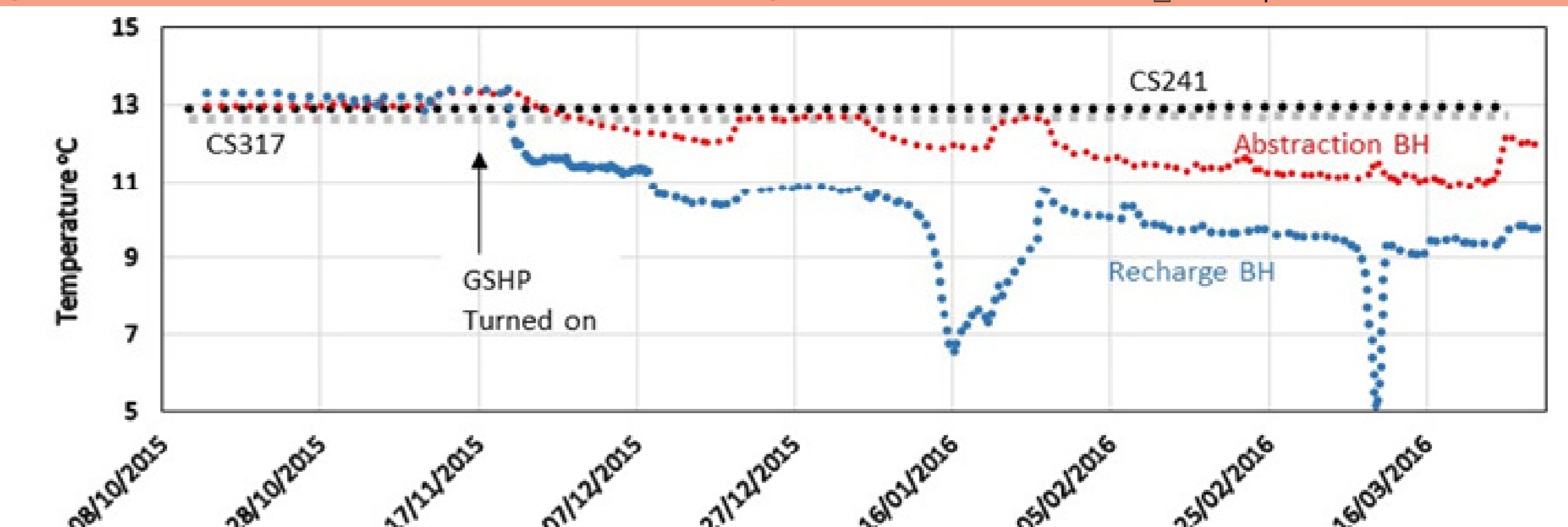
Fig. 6. Groundwater temperatures at abstraction, discharge & 2 nearby monitoring boreholes
