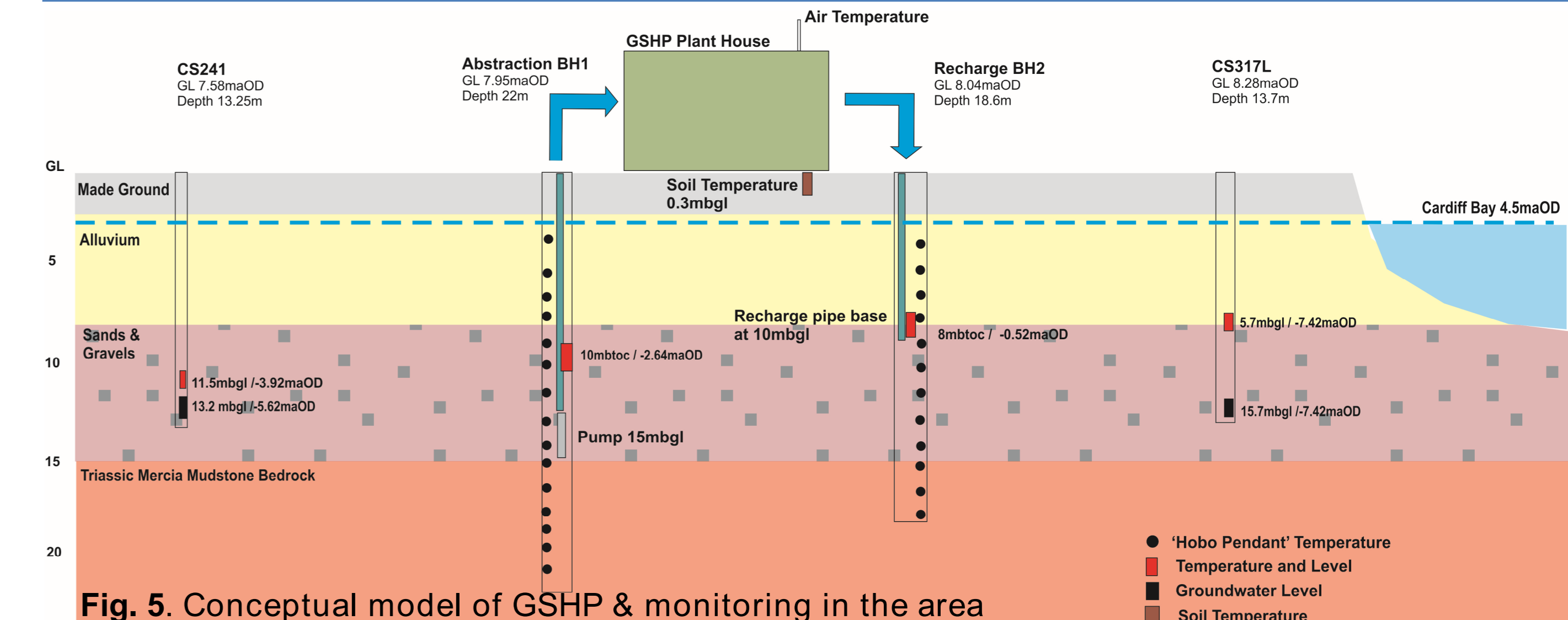
Fig. 5. Conceptual model of GSHP & monitoring in the area
