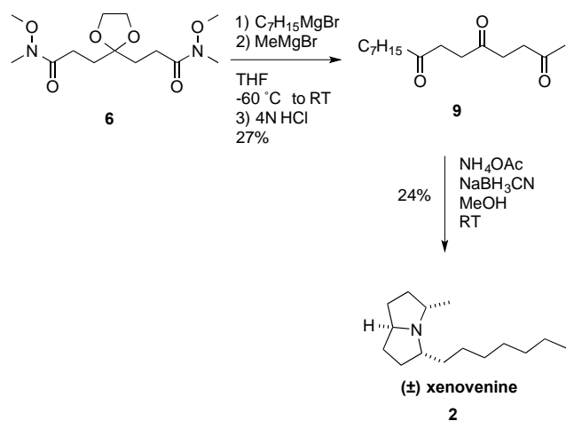
Scheme 3. Synthesis of xenovenine
