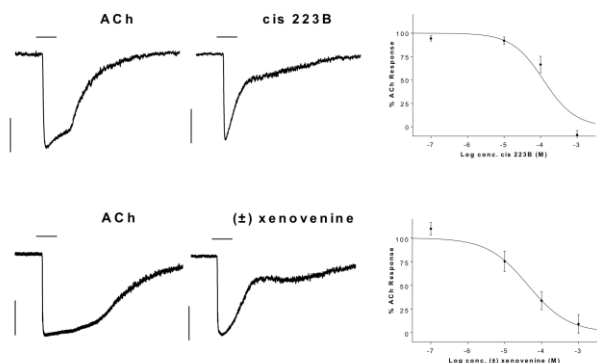
Figure 1. Inhibition of ACh (10 \mu M) induced currents in TE671 cells expressing human muscle-type nAChR by a) cis -223B and b) ( \pm )-xenovenine at V_h -75mV. Typical traces showing ACh elicited currents (left) and when co-applied with pyrrolizidines (100 \mu M)(centre). Vertical bars represent 200pA and horizontal bars show 1s perfusion period. Concentration/inhibition plots fitted with non-linear regression curves. The current at 1s after onset (the point at which antagonism is greatest) was normalised against the preceding ACh only response at the same time point. Values represent mean \pm SEM for 5-12 cells.
