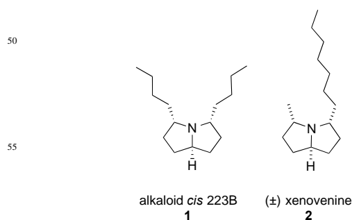
Figure 1. Structures of alkaloid cis -223B and xenovenine
