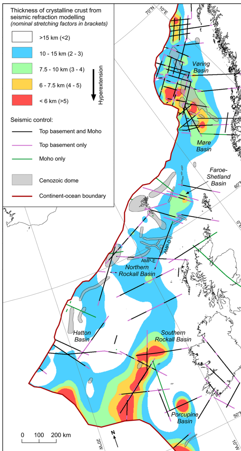
Fig. 3. Thickness of crystalline crust on the NW European margin based on the seismic refraction compilation of Funck et al. (2014, this volume, in press). Nominal stretching factors are based on an initial crustal thickness of 30 km (see the text).
