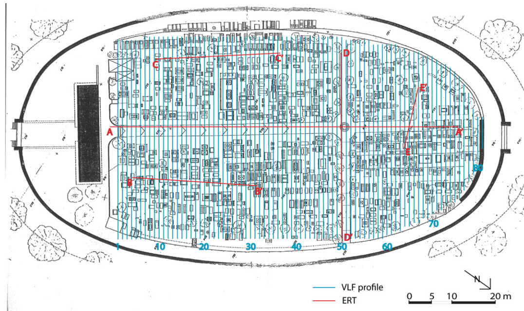
Fig. 5. Plan of the English Cemetery with location of the 82 VLF-EM profiles (blue lines) and the 5 2D-ERTs (red lines).
