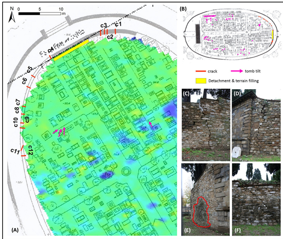
Fig. 11. (A) Crack pattern map onto the Karous-Hjelt filtered in-phase component of the VLF-EM survey of the northern sector of the English Cemetery, where fractures mainly concentrate compared with the (B) distribution of the observed tomb tilts. Detailed views of cracks (C) c3 and (D) c4 close to the monumental niche; (E) wet area (red line) over the exterior surface of the wall close to crack c3. (F) Crack c11 diagonally runs along the western wall (photo credit D. Tapete).
