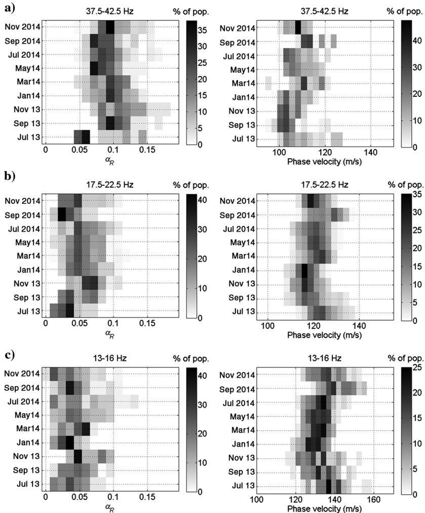
Figure 8. Overall distribution of Rayleigh-wave attenuation coefficients ( \alpha_R , left column) and phase velocities (right column) from the July 2013 to November 2014 data sets for three frequency bands: (a) 37.5–42.5 Hz, (b) 17.5–22.5 Hz, and (c) 13–16 Hz corresponding to the pseudodepths of 1.5, 3, and 4.5 m, respectively. The gray scale refers to the percentage of \alpha_R /velocities falling in a particular histogram bin over the population of attenuation coefficients/phase velocities comprised in the considered frequency band.
