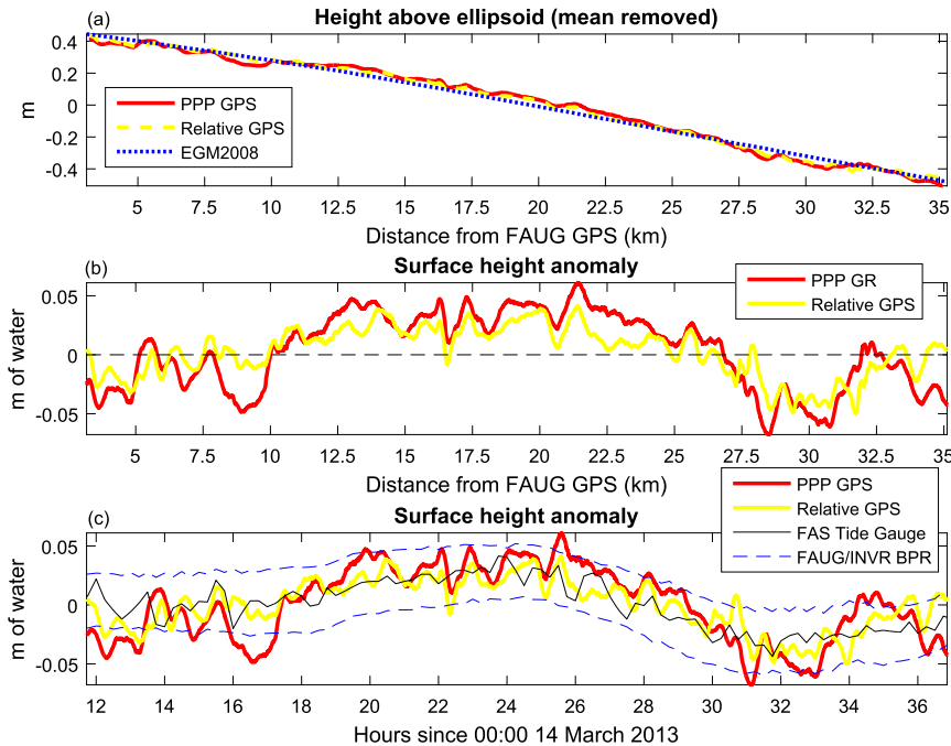
FIG. 4. (a) Kinematic PPP (red) and relative (yellow) 900-s GPS ellipsoidal heights against distance from FAUG GPS station ( 57^{\circ}08'09.6''N , 4^{\circ}41'16.8''W ). Also shown are the EGM2008 (blue) geoid heights, plotted with the mean removed. (b) Surface height anomalies: Kinematic PPP GPS 900-s ellipsoidal minus EGM2008 geoid heights (red) and relative 900-s GPS ellipsoidal minus EGM2008 geoid heights (yellow) as a function of linear distance from FAUG GPS station. (c) Surface height anomalies: Kinematic PPP GPS 900-s ellipsoidal minus EGM2008 geoid heights (red) and relative 900-s GPS ellipsoidal minus EGM2008 geoid heights (yellow) as a function of time. Also shown are the 900-s time series of surface height from the FAS tide gauge (black) and the equivalent surface height derived from the FAUG BPR (offset by 0.025 m; dashed blue curve top) and INVR BPR (offset by -0.025 m; dashed blue curve bottom). The mean values have been removed from all the time series.
