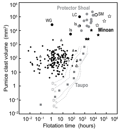
Figure 14. Flotation time of cold pumice from this study compared with published literature. The pumice from the studied unit (black diamonds) sank much faster than ~90% of the Taupo pumice clasts and did not follow the same rate of waterlogging with clast volume. Pumice lapilli from U1396A-8H2, 104 cm (open gray triangles), and other pumice clasts from U1396A-8H2, 8H3, 9H4 and 9H5 (filled gray triangles; see text), interpreted as rafted pumice clasts, share similarities with the pumice from the stratified pumice lapilli-ash and with the Taupo pumice. Symbols: gray squares and dashed gray percentiles lines—Taupo Plinian (A.D. 232 eruption; New Zealand; White et al., 2001; Hogg et al., 2012); gray dots—Protector Shoal (1962 eruption in the Sandwich Islands, sub-Antarctica; Risso et al., 2002); black and open (inferred data) stars—Minoan Plinian (1500 B.C. eruption at Santorini, Greece; Whitham and Sparks, 1986); WG—W-tephra (Guatemala; Whitham and Sparks, 1986); Is—Ischia (San Angelo, Italy; Whitham and Sparks, 1986); LC—Los Chocoyos (Guatemala; Whitham and Sparks, 1986); SM (inferred data)—Santa Maria (Guatemala; Whitham and Sparks, 1986).
