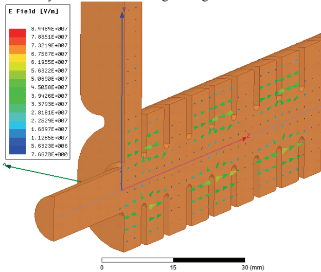
Figure 2: Shows the input coupler and the first 9 cells of the un-damped crab cavity prototype. The electric field is plotted for an input power of 13.35 MW.
