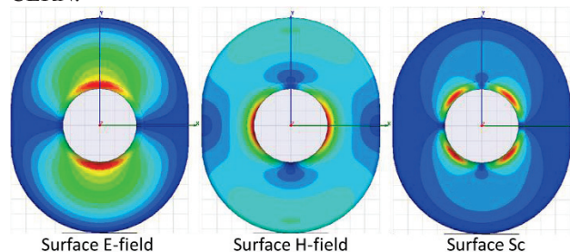
Figure 1 shows the cell geometry and the E-field, H-field and the modified pointing vector 'Sc' [3] of the un-damped crab cavity as simulated in HFSS.
