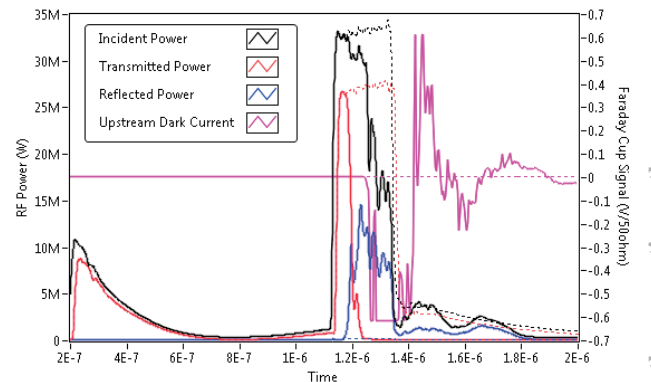
Figure 3: shows a normal compressed pulse (dotted lines) and a breakdown pulse (solid lines) inside the crab cavity.
