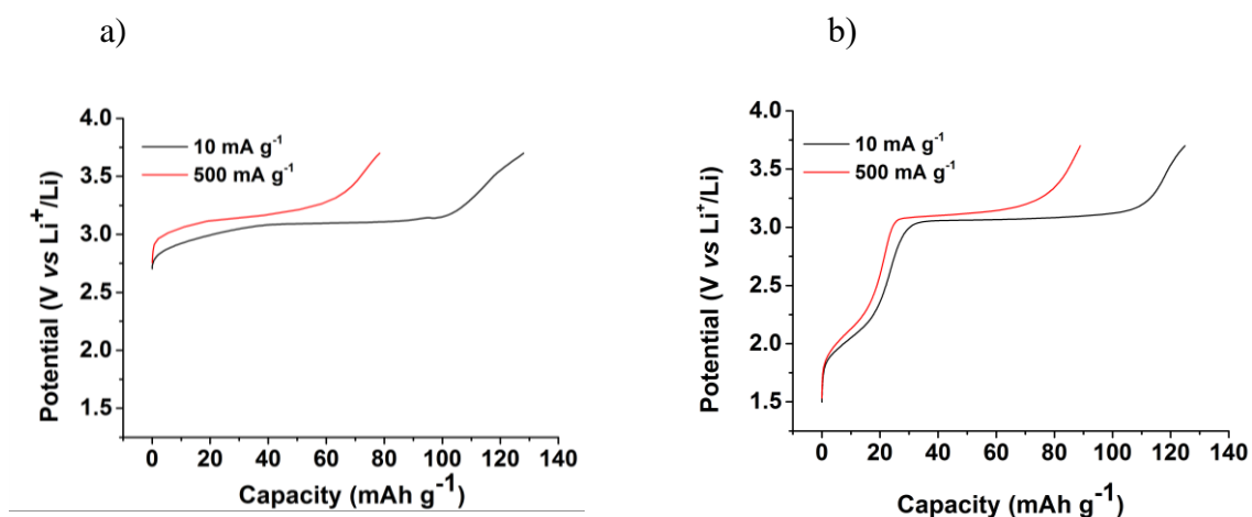
Figure 6. Load curves for a) \text{Li}_2\text{FeSiO}_4 and b) \text{Li}_{2.6}\text{Fe}_{0.7}\text{SiO}_4 obtained at 10 and 500 \text{mA g}^{-1} during the 1 st cycle
