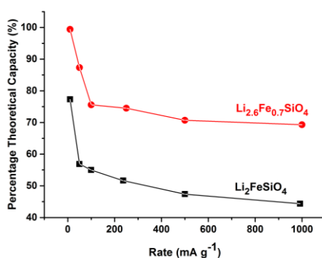
Figure 5. Percentage of theoretical capacity as a function of the discharge rate. Each capacity was determined from the first charge of a freshly assembled cell such that at the start of charge the \text{Li}_2\text{FeSiO}_4 was \gamma_s and \text{Li}_{2.6}\text{Fe}_{0.7}\text{SiO}_4 was \gamma_{II}
