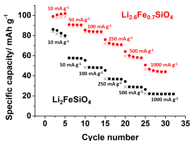
Figure 8. Charge and discharge capacity at a series of different rates for both \text{Li}_2\text{FeSiO}_4 and \text{Li}_{2.6}\text{Fe}_{0.7}\text{SiO}_4 at room temperature.
