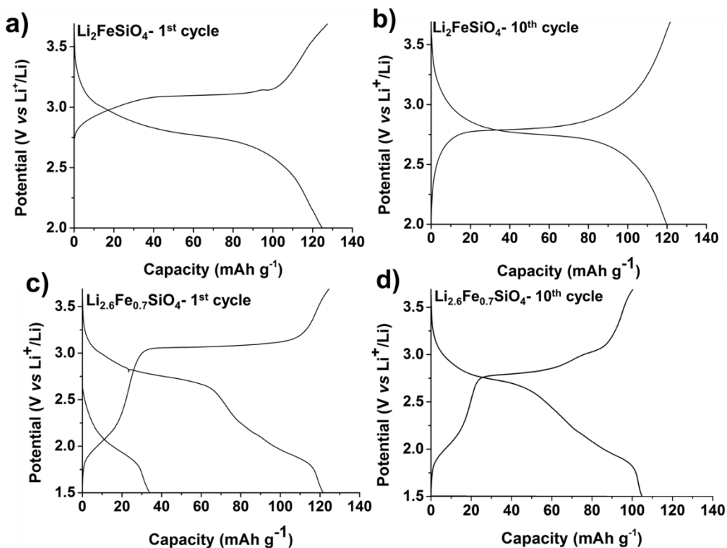
Figure 3. Load curves for as-prepared \text{Li}_2\text{FeSiO}_4 cycled between 2.0 and 3.7 V at 10 \text{ mA g}^{-1} and 60^\circ \text{C} on the 1 st cycle (a); and 10 th cycle (b). Load curves for as-prepared \text{Li}_{2.6}\text{Fe}_{0.7}\text{SiO}_4 cycled between 1.5 and 3.7 V (starting with a discharge to insert Li interstitials) at 10 \text{ mA g}^{-1} and 60^\circ \text{C} on the 1 st cycle (c); and 10 th cycle (d)
