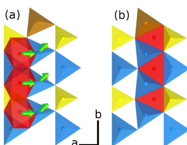
Figure 13. Transport mechanism of the Li-rich cluster in \text{Li}_{2.6}\text{Fe}_{0.7}\text{SiO}_4 ; (a) initial configuration (b) after migration. Key: octahedral interstitial Li ions (red), tetrahedrally coordinated Li (blue), Fe (brown) and Si (yellow). Arrows indicate the migration pathways of lithium ions between face-sharing octahedral and tetrahedral sites via a cooperative knock-on mechanism.
