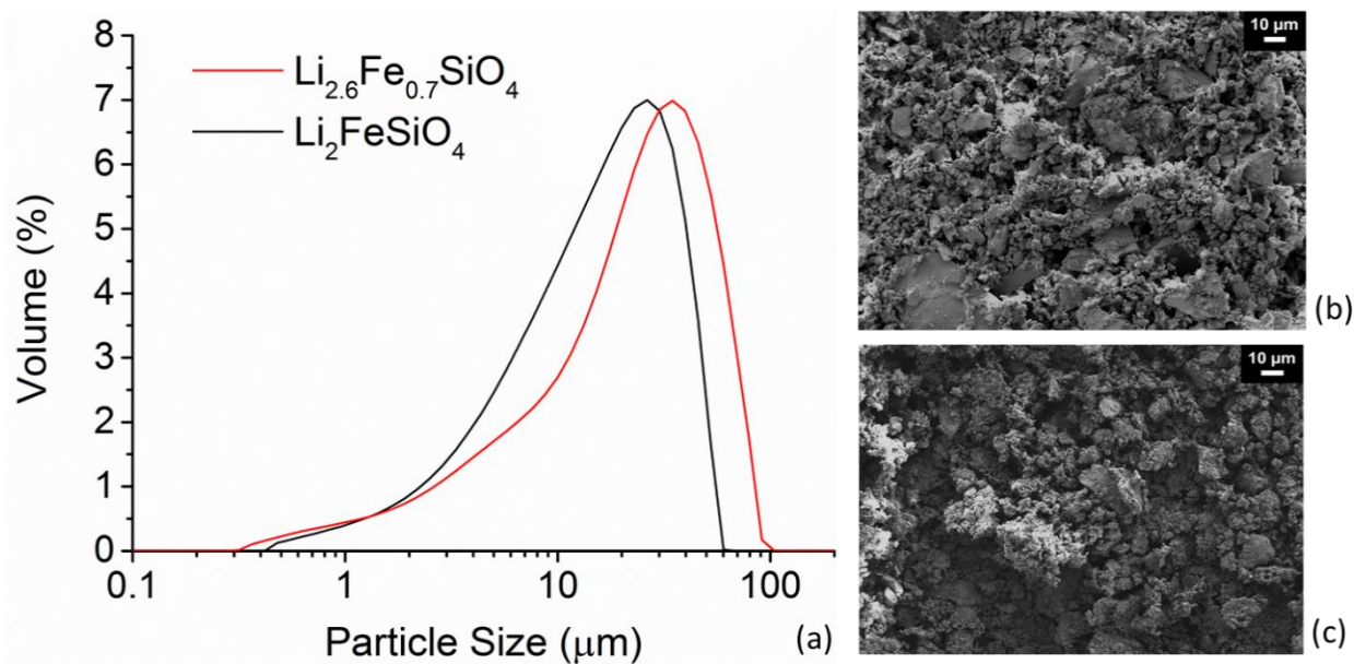
Fig. S2 a) Particle size distributions for as-prepared \text{Li}_{2+2x}\text{Fe}_{1-x}\text{SiO}_4 materials. SEM (secondary electron, 2 kV accelerating voltage, 500X magnification) images of as-prepared \text{Li}_{2+2x}\text{Fe}_{1-x}\text{SiO}_4 materials. b) x = 0 and c) x = 0.3 .
