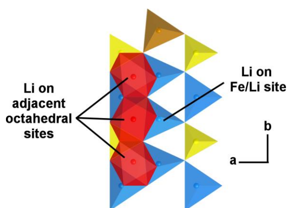
Figure 9. Typical lithium-rich defect cluster in \text{Li}_{2.6}\text{Fe}_{0.7}\text{SiO}_4 in which lithium occupies adjacent octahedral sites and shared Li/Fe tetrahedral sites. Octahedral interstitial Li ions are shown in red, tetrahedrally-coordinated Li, Fe and Si are shown in blue, brown and yellow, respectively
