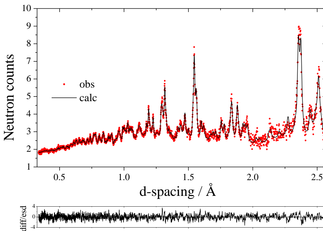
Fig. S5 Profile fit to neutron diffraction data for Li 2.6 Fe 0.7 SiO 4 discharged to 1.5V. The observed (●) and calculated (—) patterns are shown; and the difference/esd is shown in the lower panel.
