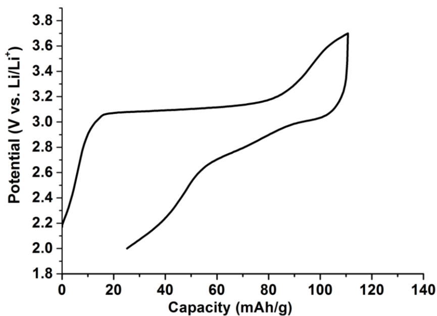
Fig. S3 Load curve for as-prepared \text{Li}_{2.6}\text{Fe}_{0.7}\text{SiO}_4 cycled between 2.0 and 3.7 V at 10 \text{mA g}^{-1} and 60 °C.
