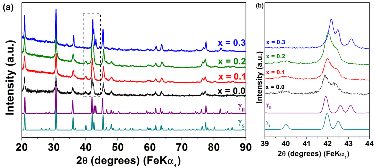
Figure 2. a) Powder X-ray diffraction patterns for the as-prepared \text{Li}_{2+2x}\text{Fe}_{1-x}\text{SiO}_4 materials ( 0 \leq x \leq 0.3 ) and reference patterns for \text{Li}_2\text{FeSiO}_4 in the P2_1/n ( \gamma_s ) and Pmnb ( \gamma_{\text{II}} ) space groups. b) XRD patterns in the selected region of 39 - 44^\circ 2\theta
