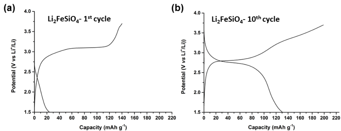
Fig. S4 Load curve for as-prepared Li 2 FeSiO 4 cycled between 1.5 and 3.7 V at 10 mA g -1 and 60 °C. This cycling range caused a rapid capacity fade and change to the voltage profiles observed.
