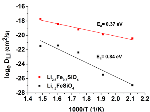
Figure 11. Arrhenius plot of lithium diffusion coefficients D_{\text{Li}} of \text{Li}_{2-x}\text{FeSiO}_4 ( x=0.2 ) and \text{Li}_{2.6}\text{Fe}_{0.7}\text{SiO}_4 with derived activation barriers ( E_a )
