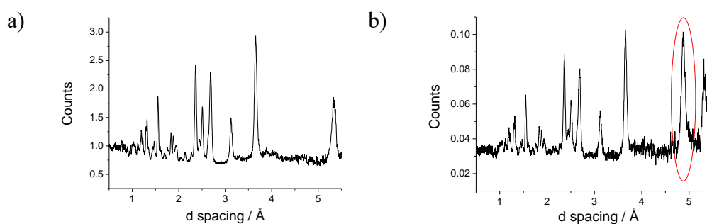
Figure 4. Powder neutron diffraction patterns (Polaris Bank 3) for a) as-prepared \text{Li}_{2.6}\text{Fe}_{0.7}\text{SiO}_4 , b) \text{Li}_{2.6}\text{Fe}_{0.7}\text{SiO}_4 discharged to 1.5V with the superlattice reflection highlighted
