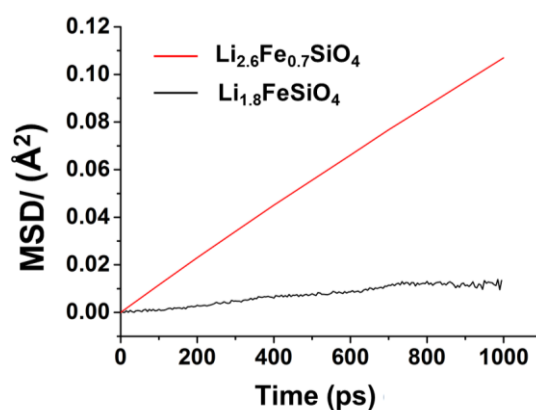
Figure 10. Mean squared displacement (MSD) of lithium ions vs time at 573 K comparing \text{Li}_{2.6}\text{Fe}_{0.7}\text{SiO}_4 to \text{Li}_{2-x}\text{FeSiO}_4 [ x = 0.2 ]. The total simulation time was 3 ns and the final 1 ns is shown here.
