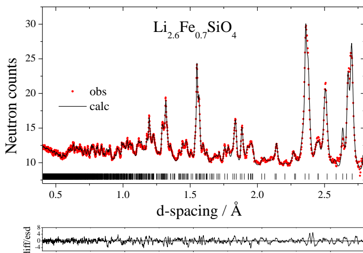
Figure S1 Profile fits to neutron diffraction data for as-prepared \text{Li}_{2+2x}\text{Fe}_{1-x}\text{SiO}_4 materials. a) x = 0.1 , b) x = 0.2 and c) x = 0.3 . The observed ( \bullet ) and calculated ( \text{---} ) patterns are shown; and the difference/esd is shown in the lower panel.
