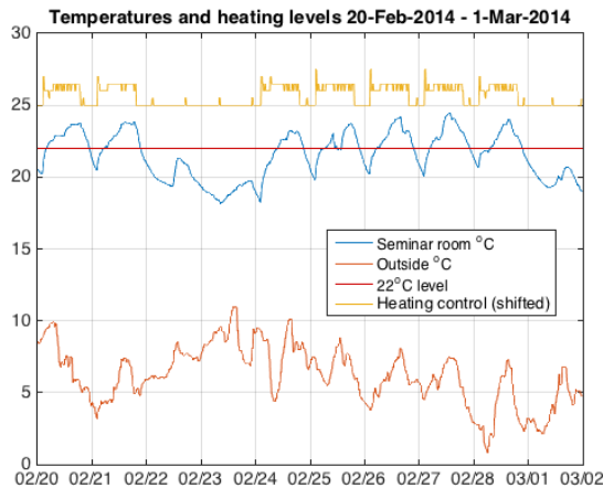
Fig. 2. Temperature and heating input to a seminar room from historical data used to create a new control schedule to avoid overheating and trim heating to occupied hours.
