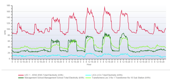
Fig. 1. Top level energy use for 3 department buildings, April 4-12 2015. Weekdays clearly exhibit higher peaks than weekends. Substantially different baseline loads are also obvious, but load is not normalised by building size or occupancy.
