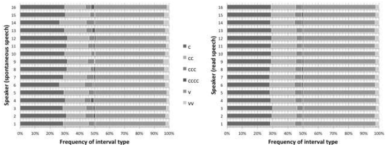
Figure 3: Stacked bar-chart showing the relative frequency of interval types for each speaker (rows) in spontaneous (left) and read speech (right).
