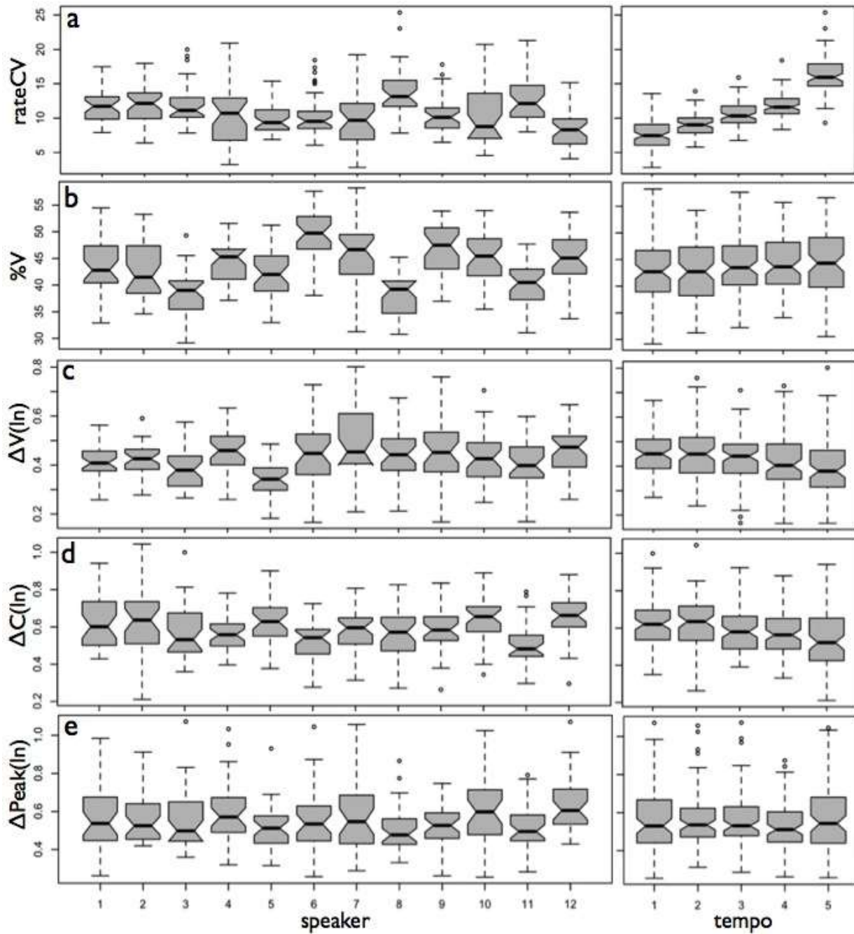
Figure 1: Boxplots showing the distributions of the variables (a) rateCV, (b) %V, (c) \Delta V(\ln) , (d) \Delta C(\ln) and (e) \Delta \text{Peak}(\ln) as a function of speaker (left ) and of intended tempo (right).
