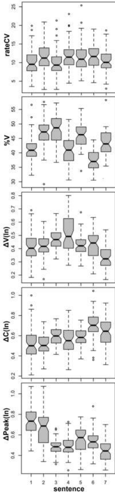
Figure 2: Boxplots showing the distributions of each of the variables under investigation (rateCV, %V, \Delta V[\ln] , \Delta C[\ln] , \Delta \text{Peak}[\ln] ) for the seven different sentences.
