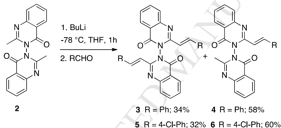
Scheme 2 Synthesis of 2,2'-styryl 3-4 , and p -chlorostyryl BiQs 5-6
