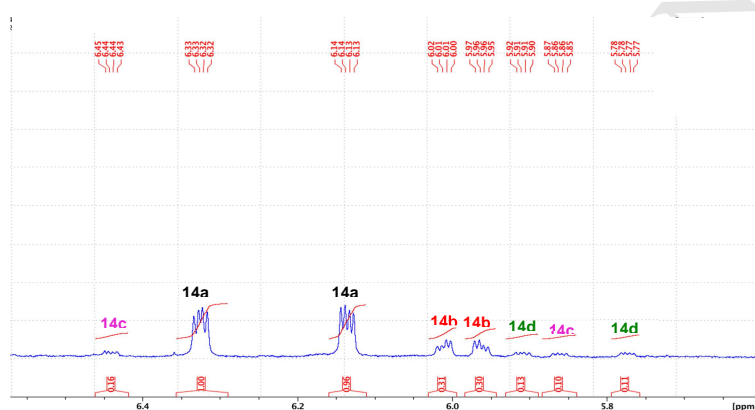
Figure 4 Expansion of the ^1\text{H-NMR} spectrum (500 MHz, \text{CDCl}_3 ) of the crude reaction mixture between compound 3 and cyclopentadiene.
