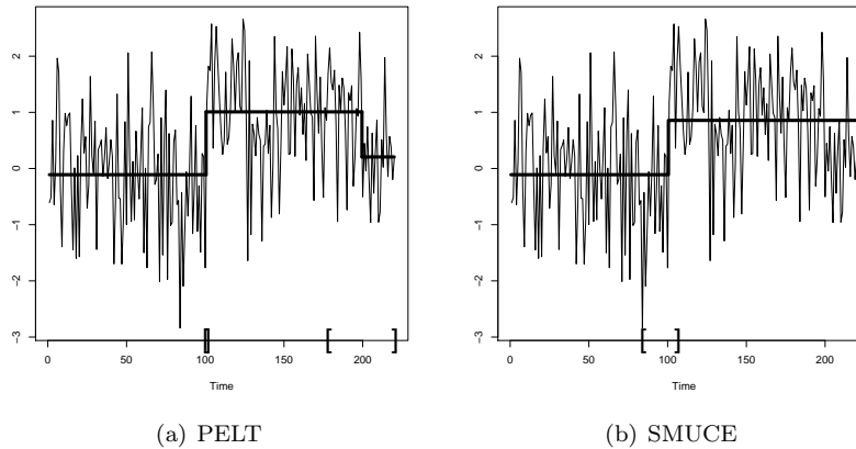
Figure 1: Simulated data with two changes in mean at 100 and 200 with (a) PELT and (b) SMUCE changepoints estimates and confidence intervals.
